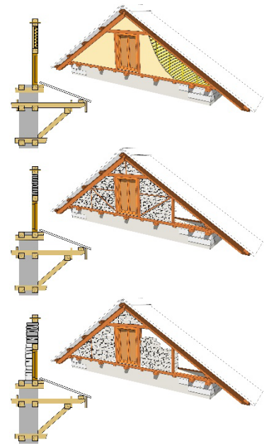
Options for lightweight gable walls: wattle and daub, or thin confined stone masonry – ©CRAterre
