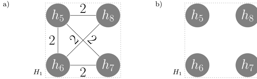
Fig. 6. Removing arcs from a induced graph. a) Induced graph \langle H_1, E|_{\neq 3} \rangle b) Induced graph \langle H_1, E|_{=1} \rangle .
