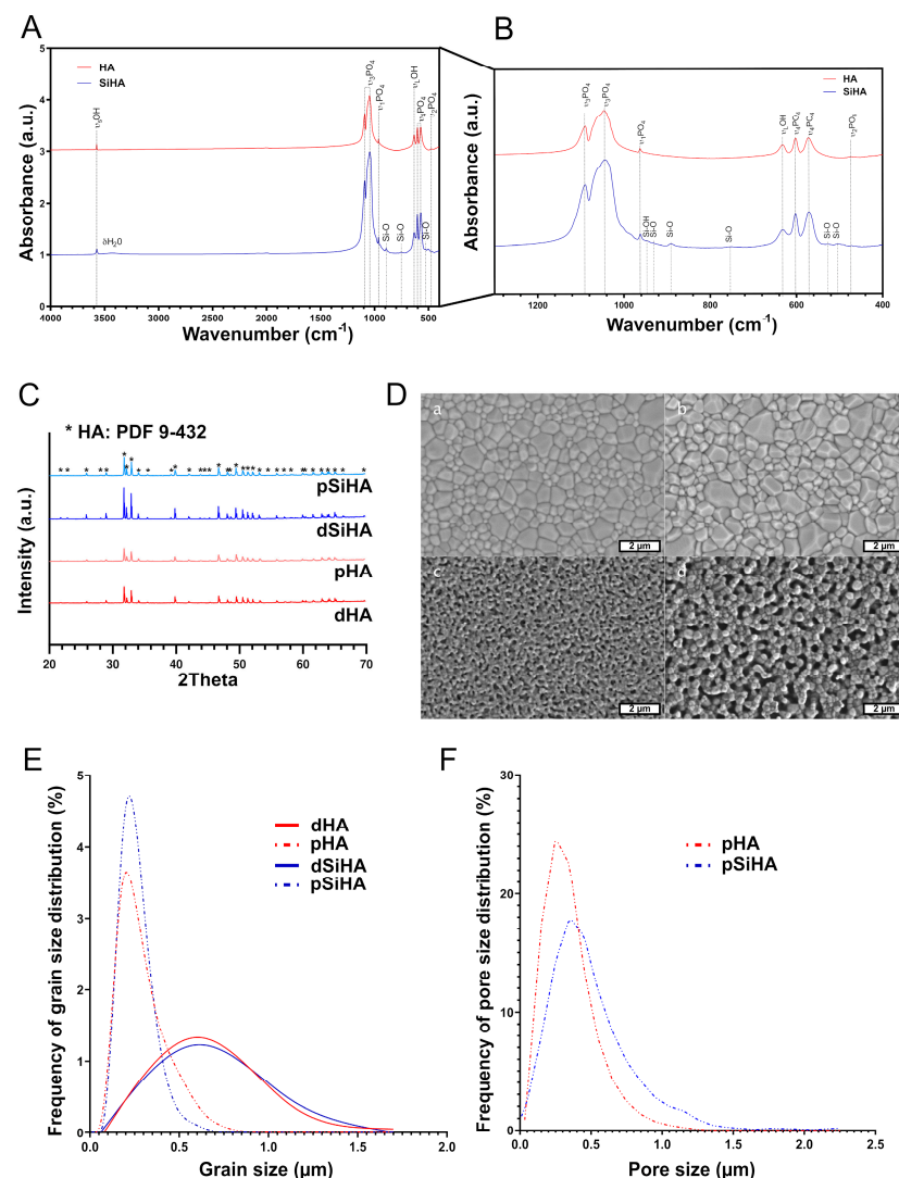
Figure 1. Chemical–physical characterization of HA-based ceramics. (A) FTIR analysis of the HA powders. (B) Inset of FTIR spectra of the HA powders from 400 to 1250 \text{ cm}^{-1} . (C) XRD diffractograms of the sintered ceramic pellets indexed according to ICDD-PDF card n°9-432 (*). Microstructure of HA-based ceramics. (D) Scanning electron microscopy micrograph of the surface of the ceramic pellets: (a). dense HA; (b). dense SiHA; (c). porous HA; and (d). porous SiHA. Scale bar (white): 2 \mu\text{m} . (E) Distribution frequency of the grain size. (F) Distribution frequency of the pore size.
