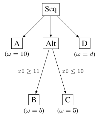
(b) Control-Flow Tree of f
