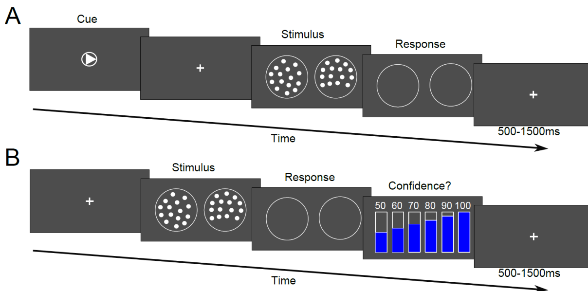
Figure 1. Experimental paradigm
