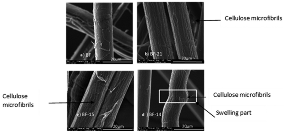
Figure 5. SEM images of fibers treated with different NaOH concentrations (a) BF (b) BF-21 (c) BF-15 and (d) BF-14.
