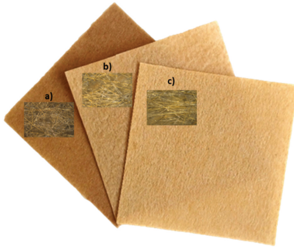
Figure 3. Pictures and optical microscopy images (x10) of BF mats treated with (a) 30%, (b) 6% and (c) 1% NaOH concentration.
