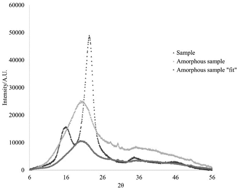
Figure 1. Crystallinity index measurement: amorphous fitting subtraction on bamboo fiber sample.
