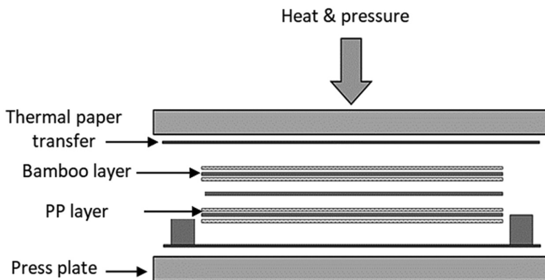
Figure 4. Composite manufacturing process.
