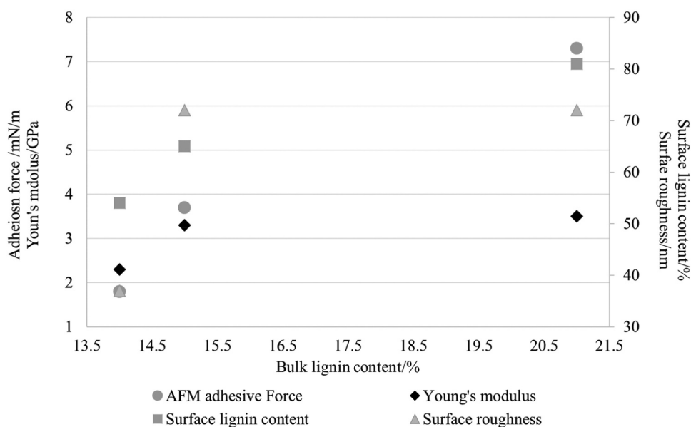
Figure 9. Evolution of the adhesion force, the young's modulus of the composites and the roughness of the fibers against the bulk lignin content.
