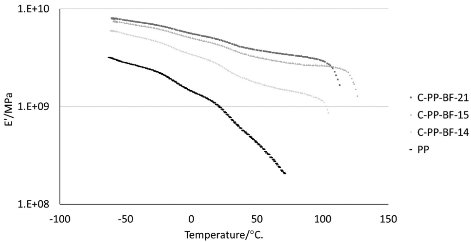
Figure 7. Evolution of the storage modulus for PP-BF composites and neat PP as a function of temperature for PP (-), PP-BF-14 (●), PP-BF-15 (▲), and PP-BF-21 (○).
