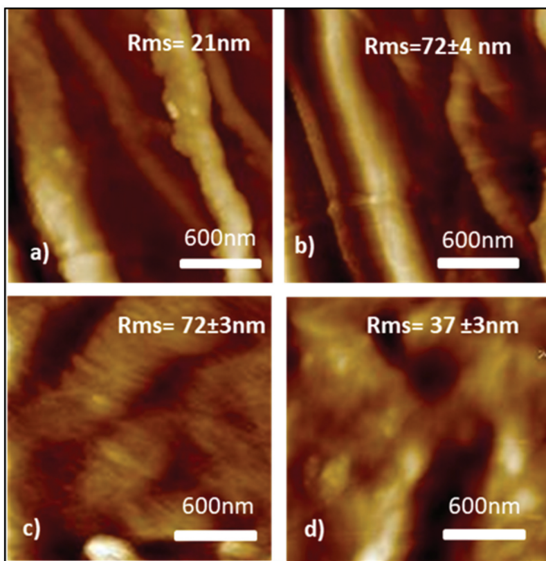
Figure 6. AFM images of fibers treated with different NaOH concentrations (a) BF (b) BF-21 (c) BF-15 and (d) BF-14.
