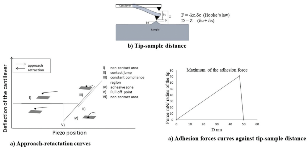
Figure 2. Principle of the adhesion measurement by AFM. (a) the approach/retraction curves (b) the tip/surface distance calculation, (c) the adhesion force versus distance after calibrations.
