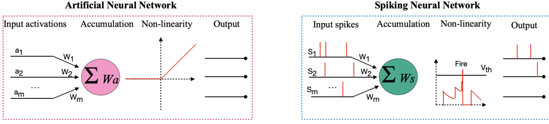
Figure 1: The structure of ANN and SNN. The ANN takes input and rectifies it if is less than 0 and passes it otherwise. The SNN takes spikes as input and fires as spikes only if the membrane potential exceeds the threshold V_{th} .
