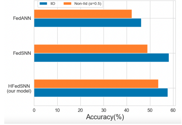
Figure 3: The classification performance (accuracy) of our model (with 5 global rounds) against FedSNN [11] and FedANN models with 40 global rounds, on IID and non-IID data with 100 clients and 10 clients participating.
