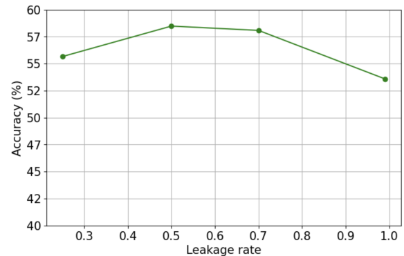
Figure 9: Classification performance with different leakage rates
