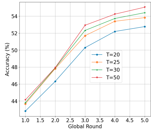
Figure 8: Performance comparison with different timesteps
