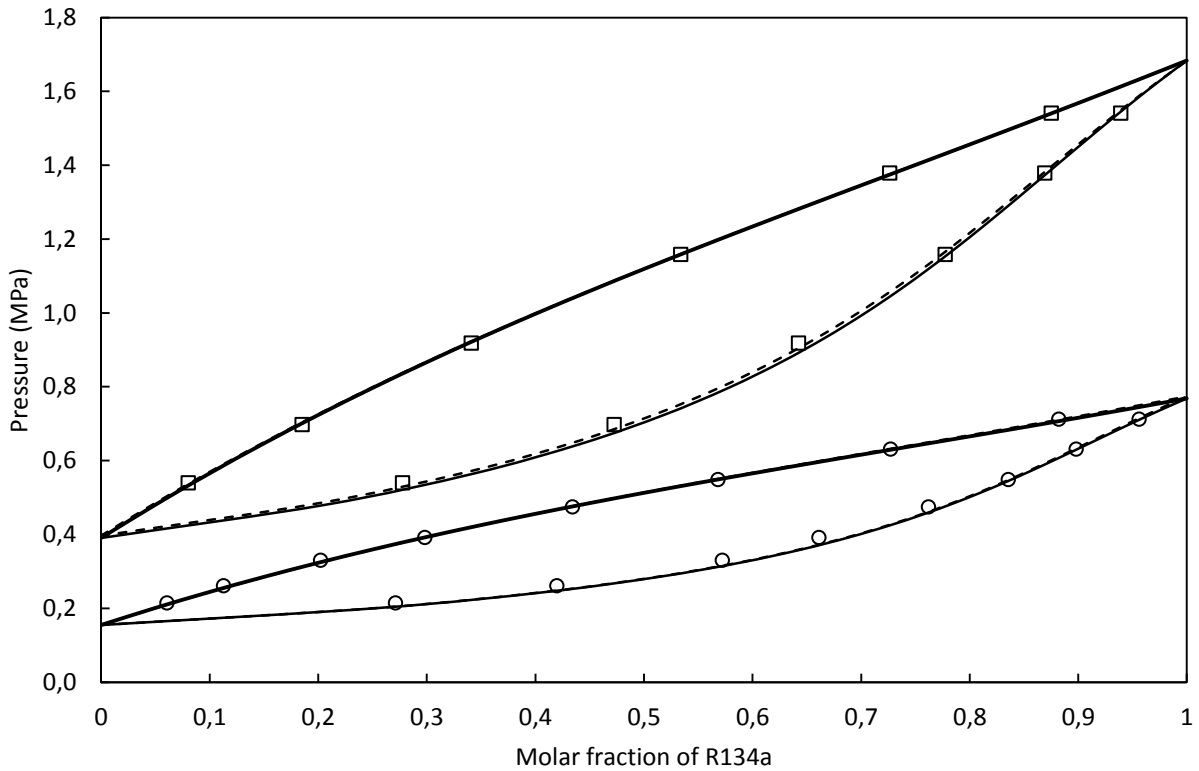
Figure 5 : P-xy phase diagram of R134a– R1233zd(E) binary system. Experimental values: 303.07 K (○) and 333.23 K (□). Modelling results: Peng-Robinson (Solid lines), NEOs (Dashed lines).
