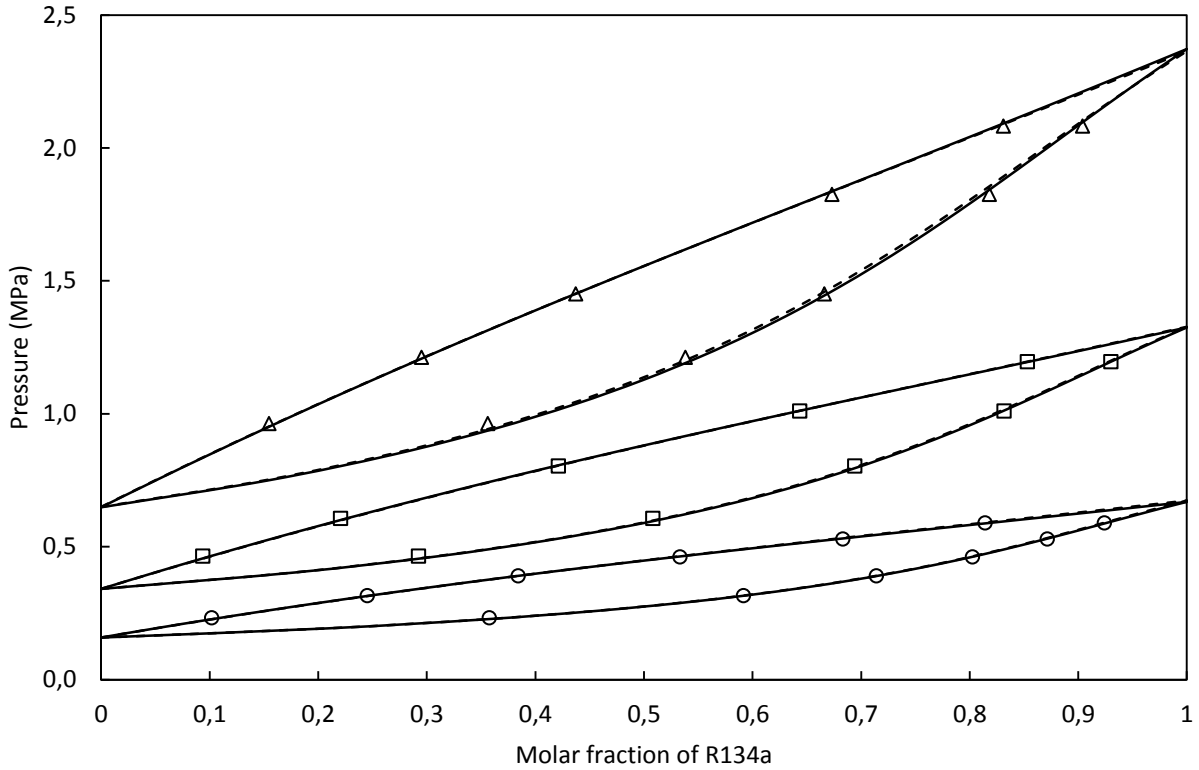
Figure 8 : P-xy phase diagram of R134a – R1233xf binary system. Experimental values: 298.30 K (○), 323.38 K (□) and 348.27 K (Δ). Modelling results: Peng-Robinson (Solid lines), NEOs (Dashed lines).
