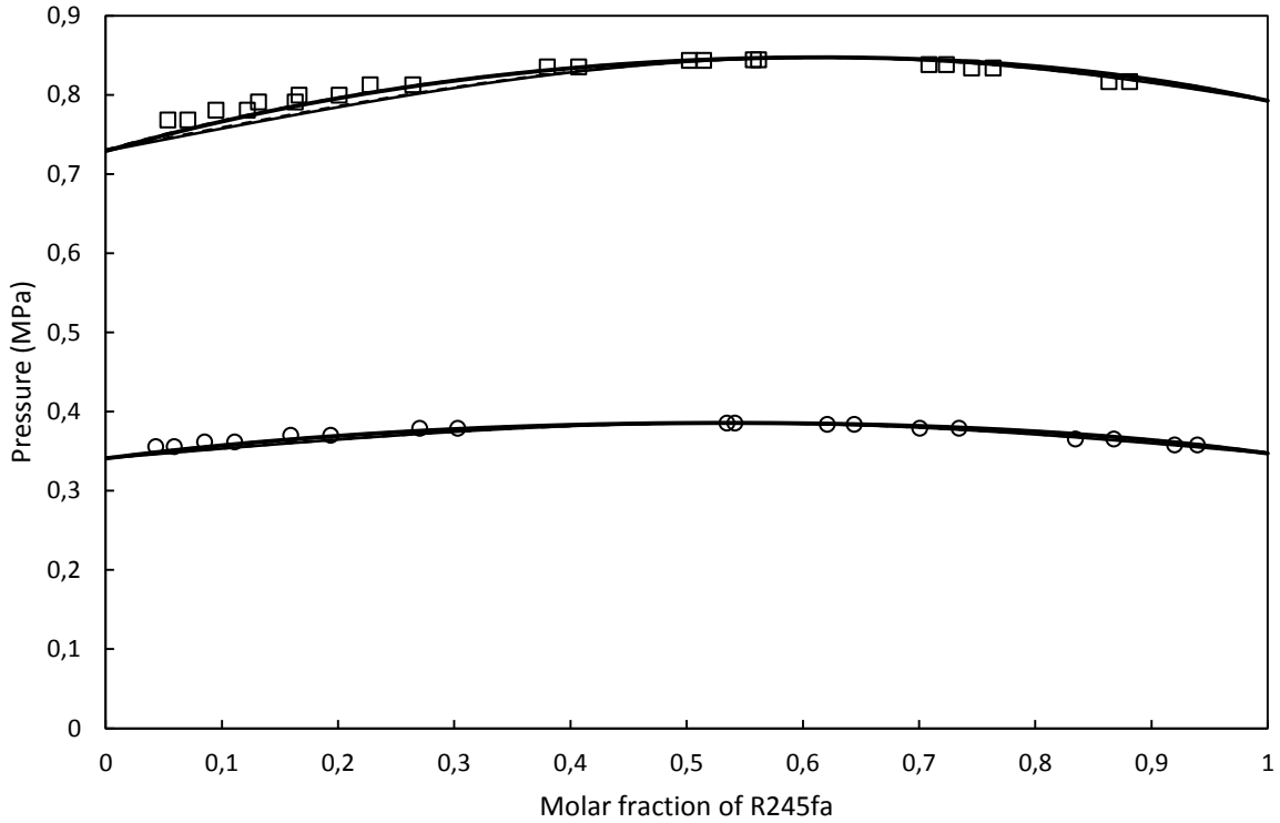
Figure 9 : P-xy phase diagram of R245fa– R1233xf binary system. Experimental values: 323.40 K (○) and 353.27 K (□). Modelling results: Peng-Robinson (Solid lines), NEOs (Dashed lines).
