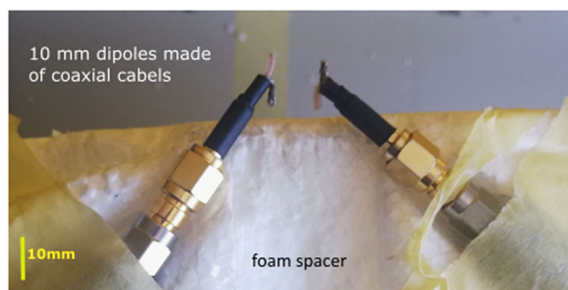
Fig. 4 Photo of the electric dipoles used in the experiments. The 10 mm dipoles are made from a coaxial cable and fixed on the foam spacer.
