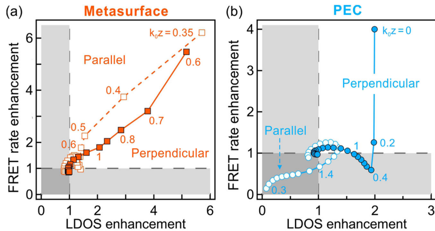
Fig. 3 The LDOS vs. FRET enhancement factor diagrams. The enhancement factor diagrams for the metasurface (a), and the plane made of perfect electric conductor (PEC) (b). The data corresponds to the experimental results of Fig. 2a–d, with a dipole–dipole distance R = \lambda/7 . Empty markers connected by dashed lines correspond to parallel dipole orientation, while filled markers and solid lines are for the perpendicular ones. The markers are shown for different heights z to the boundary, the number next to each data point indicates the normalized distance k_0 z = 2\pi z/\lambda . When the distance z increases, all the curves converge towards the free space (1,1) value.
