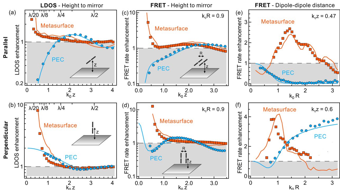
Fig. 2 The influence of surface-wave excitation on the near-field interaction processes between two dipoles. a, b Local density of states (LDOS) enhancement as a function of the height z between the plane of the dipole's center and the boundary plane for parallel ( a ) and perpendicular ( b ) orientation of the dipoles. c, d FRET rate enhancement as a function of the height z between the plane of the dipole's center and the boundary plane for the same orientation. The dipole-dipole distance is set at k_0R = 0.9 , corresponding to R = \lambda/7 . e, f FRET rate enhancement as a function of the distance R between the two dipoles. For e , the height is set at k_0z = 0.47 , corresponding to z = \lambda/14 , while for f due to the finite size of the dipoles, we switch to k_0z = 0.6 , corresponding to z = \lambda/10 . In c, e both dipoles have parallel orientation to the surface and perpendicular orientation in ( d, f ). In all the graphs, markers correspond to experimental data while lines are numerical calculations. The technical error associated with measurements is described in the “Methods” section.
