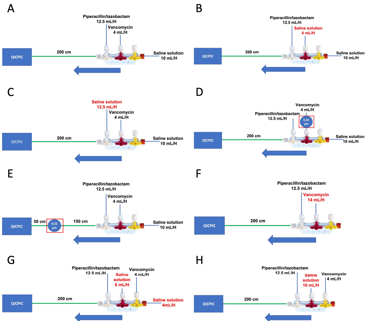
Figure 2. The standard manifold infusion set (A), the vancomycin solution replaced by SS (B), the piperacillin/tazobactam solution replaced by SS (C), the manifold infusion set with a filter on the vancomycin solution tubing (D), the manifold infusion set with a filter on the tubing downstream of the tap manifold (E), the manifold infusion set with diluted vancomycin (F), the manifold infusion set with two SS administration routes (G), and the manifold infusion set with an SS alternative administration route (H).
