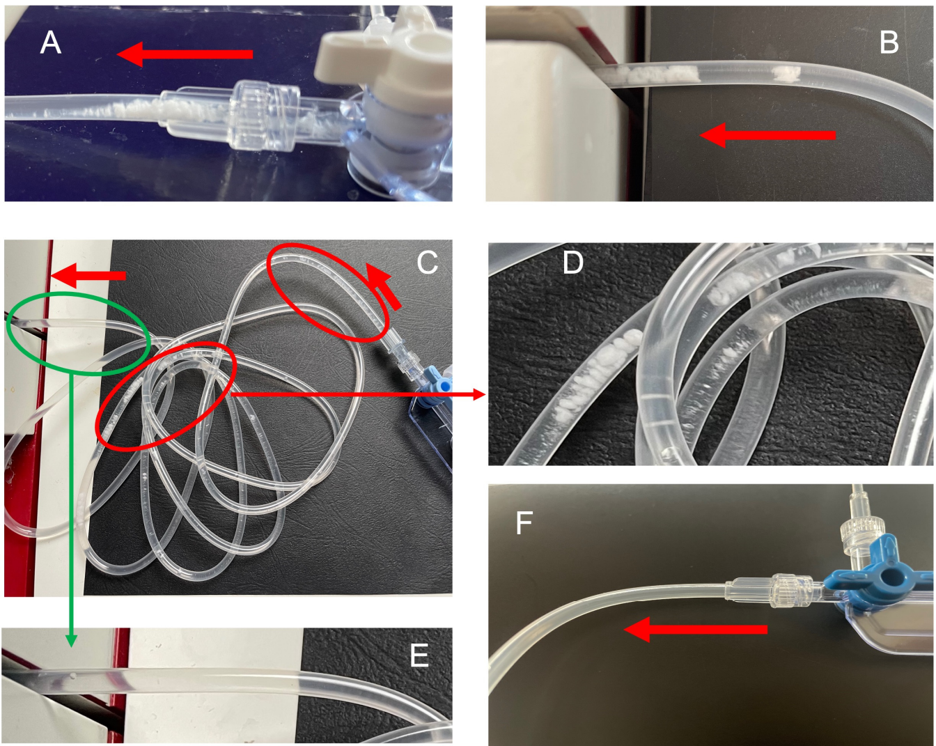
Figure 3. Visual observation of the infusion lines. The red arrows indicate the direction of infusion. (A) Formation of the initial white precipitate, following contact between the vancomycin solution and the piperacillin/tazobactam solution. (B) The initial precipitate is only visible at the end of the infusion tubing. (C) The white precipitate dissolves along the tubing during VPT co-perfusion. The red circles (D) correspond to the presence of visible particles, and the green circle (E) corresponds to the absence of visible particles. (F) The absence of visible precipitate during a VPT co-infusion.
