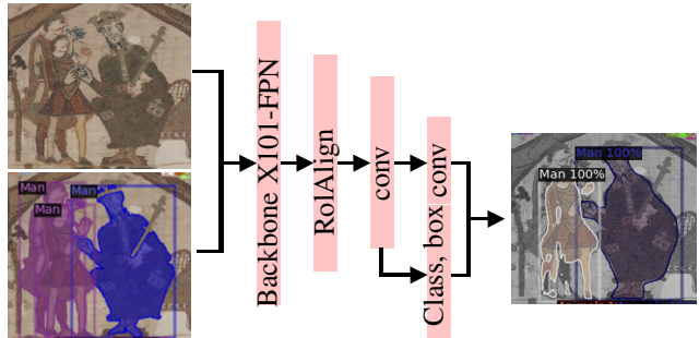
Figure 10: Mask-R-CNN neural network architecture. Pairs (images, annotations) are fed to the neural network, which is trained to locate, segment, and classify the elements present in the image. Here, segmenting the three characters is difficult, as one is partially occluded by another.
