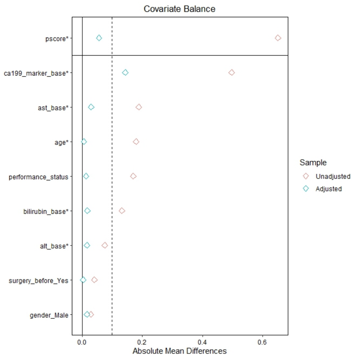
Supplementary Figure 1: Balance of the covariates between the two groups before and after adjustment using Inverse Probability of Treatment Weighting.
