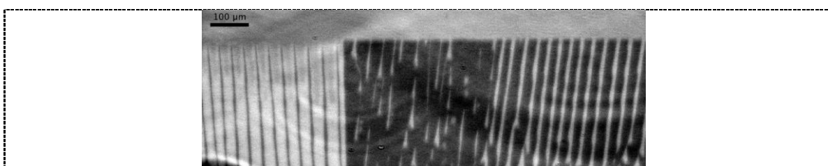
Figure 3. In situ optical observation of a lamellar pattern. Eutectic grains G3, G4 and G5, from left to right. The apparent variations of the volume phase fraction from one grain to another is related to 3D morphological features of the microstructure in the thickness of the film (see text).
