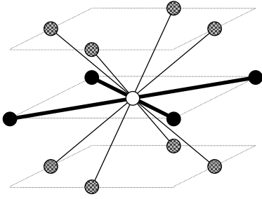
Fig. 1. First nearest neighbour shell of a Ni atom (open circle) in a face centered tetragonal structure. Each Ni atom has four first nearest neighbours in the same (001) plane (in-plane bonds) (closed circles), and eight out of this plane (out-of-plane bonds) (cross hatched circles). For a face centered tetragonal structure, the in-plane bonds are longer than the out-of-plane ones. Despite these two different distances, the twelve atoms surrounding a given Ni atom will be simply called the first nearest neighbour shell in the text.
