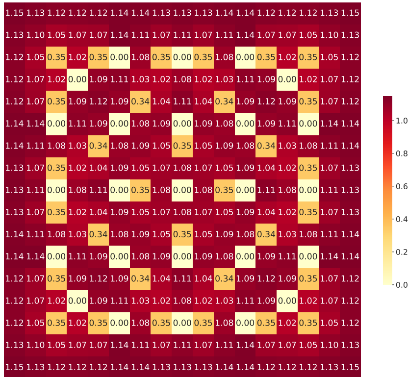
Figure 10: NYMO normalized power distribution for the PWR \text{UO}_2 fuel assembly.
