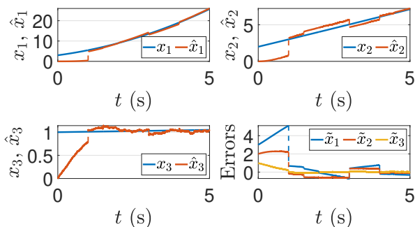
Fig. 5. State estimation in a car with multi-rate sampled outputs (with input disturbances and noise).
