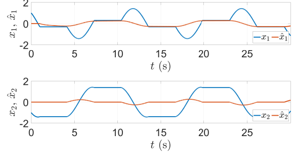
Fig. 2. State estimation in a switched system (singular switching signal).
