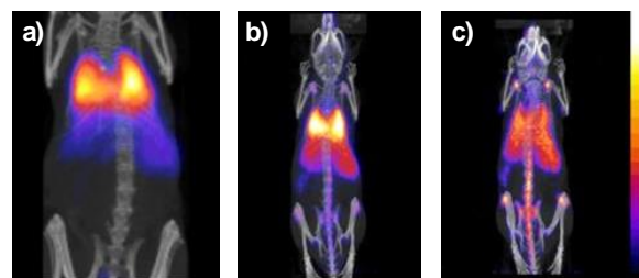
Figure 6. PET imaging after injection of ^{89}\text{Zr} -LTL-PEG into mice. Images were taken after a) 10 min, b) 18h, and c) 4d.
