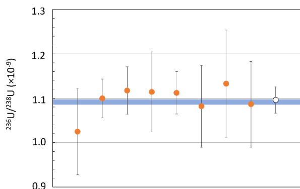
Figure 3. Measurement of ^{236}\text{U}/^{238}\text{U} isotope ratios in IRMM 075/6 certified reference material. The open dot corresponds to the mean of the measurements (red dots). The blue rectangle highlights the certified value uncertainties. Uncertainties are extended with a coverage factor of 2.
