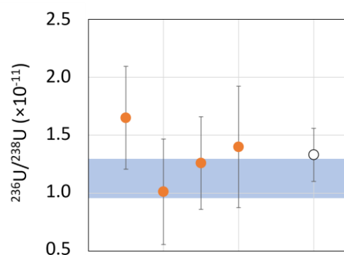
Figure 6: Measurements of ^{236}\text{U}/^{238}\text{U} isotope ratios in MTG sample. The open dot corresponds to the mean of the measurements (red dots). The blue rectangle highlights the certified value uncertainties. Uncertainties are extended with a coverage factor of 2.
