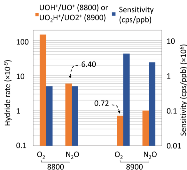
Figure 1. Comparison of the hydride formation rate and sensitivity with Agilent 8800 ICP-MS/MS (left) from Jaegler et al. (2020) and Agilent 8900 ICP-MS/MS (right) using \text{O}_2 or \text{N}_2\text{O} as a reaction gas in the CRC.
