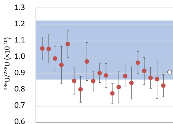
Figure 5: Measurements of ^{236}\text{U}/^{238}\text{U} isotope ratios in MBN sample. The open dot corresponds to the mean of the measurements (red dots). The blue rectangle highlights the certified value uncertainties. Uncertainties are extended with a coverage factor of 2.
