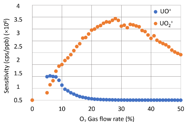
Figure 2: Uranium oxide sensitivities using oxygen in the CRC, measured as \text{UO}^+ (blue) or \text{UO}_2^+ (orange).
