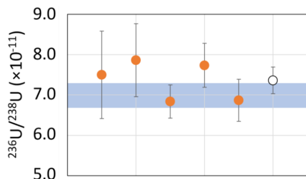
Figure 4: Measurement of ^{236}\text{U}/^{238}\text{U} isotope ratios in KkU reference material. The open dot corresponds to the mean of the measurements (red dots). The blue rectangle highlights the certified value uncertainties. Uncertainties are extended with a coverage factor of 2.
