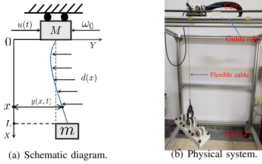
Fig. 1: The gantry crane system: schematic diagram and physical system.
