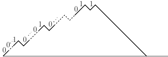
FIGURE 4. Bijection between \mathcal{L} and binary words avoiding consecutive 1s except the tail 011.
