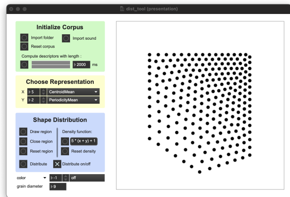
Figure 4. Screenshot of a Max patch demonstrating polyspring capabilities. The user can draw custom regions directly on the visualizer and type any density function of x and y such as \rho(x, y) = 5(x + y) + 1 .
