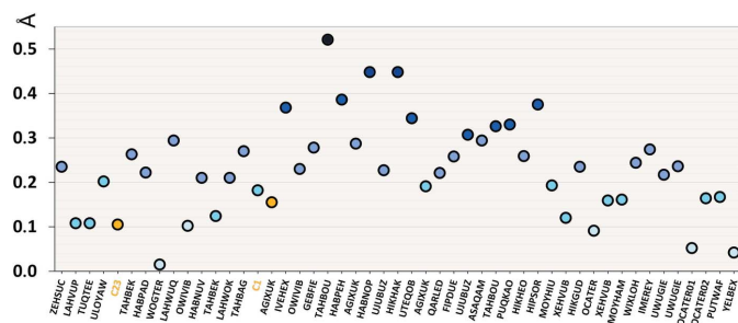
Figure 7 Delta values (blue) of ortho -carborane \text{CH}\cdots\pi\text{C}_6 contact distances defined as \Delta = d_{\text{max}} - d_{\text{min}} . The experimental values for C1 and C23 are highlighted in orange.
