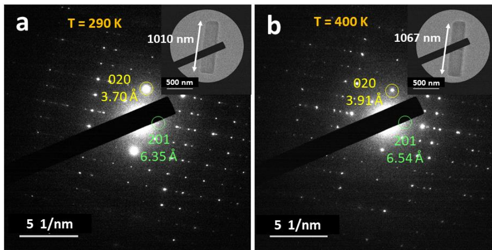
Figure 3: Diffraction patterns and images (insets) of a [\text{Fe}(\text{Htrz})_2\text{trz}](\text{BF}_4) crystal showing the lattice expansion (diffraction) and the size expansion (imaging) in the transformation from the low-spin (290 K) to the high-spin (400 K) phases of the same SCO particle. The maximum lattice expansion occurs in the b-direction.
