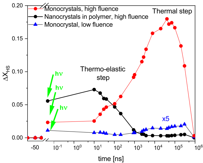
FIG. 1. Photoconversion to femtosecond laser excitation of LS [\text{Fe}^{\text{III}}(3\text{-MeO-SalEen})]\text{PF}_6 in the form of micro- and nanocrystals. “ h\nu ” denotes the photoinduced step, followed by thermoelastic and thermal steps.
