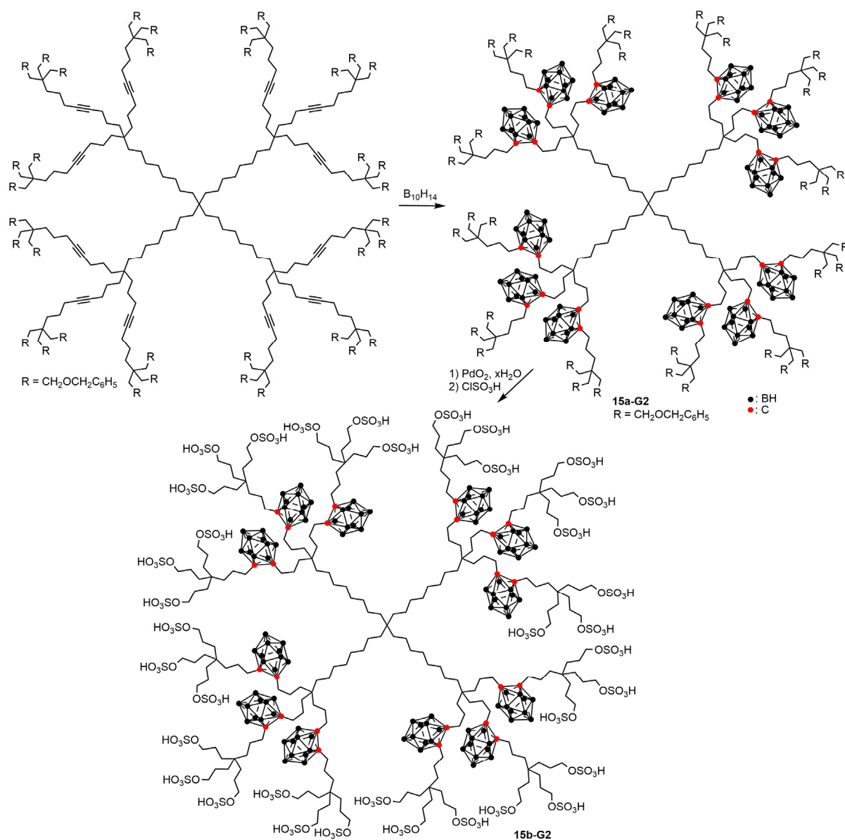
Scheme 15. Addition of decaborane to internal alkyne of hydrocarbon dendrimers, and subsequent transformation of the terminal functions to obtain a water-soluble dendrimer.
