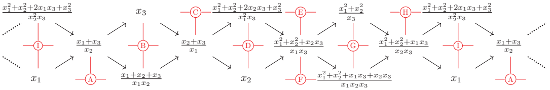
FIGURE 8 The facet-defining inequalities of the type cone \mathbb{T}\mathbb{C}(\mathcal{F}(B_\circ)) of the cluster fan correspond to the mesh mutations described in Theorem 2.23. See Section 3 for a representation theoretic interpretation.
