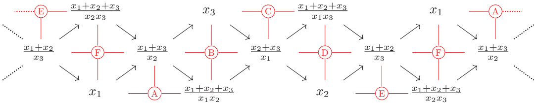
FIGURE 7 The facet-defining inequalities of the type cone \mathbb{T}\mathbb{C}(\mathcal{F}(B_\circ)) of the cluster fan correspond to the mesh mutations described in Theorem 2.23. See Section 3 for a representation theoretic interpretation.
