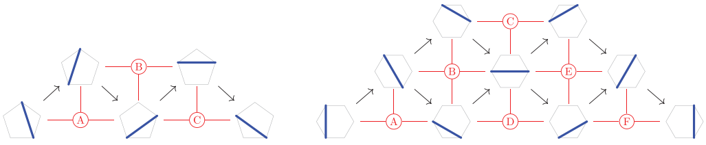
FIGURE 5 The facet-defining inequalities of the type cone \mathbb{T}C(\mathcal{F}(n)) correspond to the flips described in Proposition 2.6. See Sections 2.2 and 3 for a representation theoretic interpretation.
