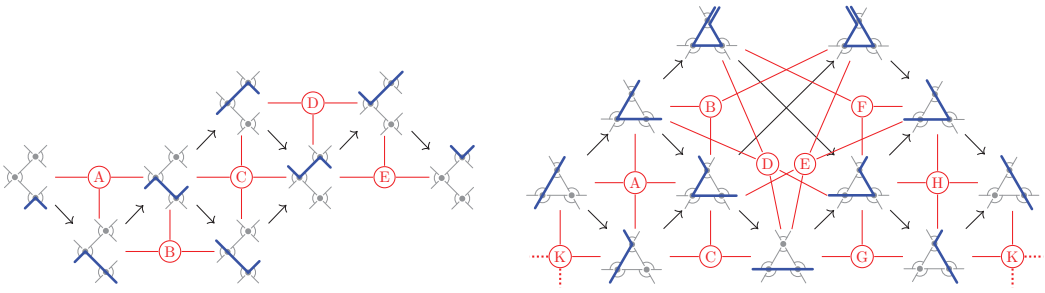
FIGURE 14 The facet-defining inequalities of the type cone \text{TC}(\mathcal{F}(\bar{Q})) of the nonkissing fan, represented on the Auslander Reiten quiver of the gentle algebra of \bar{Q} . Although they correspond to meshes on the left, they are not as clear in the general case as on the right. See also Section 4.
