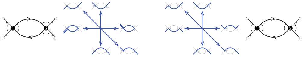
FIGURE 16 The nonkissing fans of two 2-cyclic gentle quivers. Illustration from [81].
