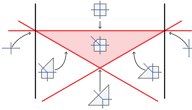
FIGURE 2 The type cone \overline{\mathbb{T}\mathbb{C}}(\mathcal{F}) of the fan \mathcal{F} of Figure 1 (left). On top of each face of \overline{\mathbb{T}\mathbb{C}}(\mathcal{F}) , we depict an example of polytope with the corresponding normal fan.
