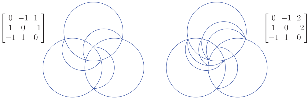
FIGURE 6 Two cluster fans \mathcal{F}(B_o) for the type A_3 (left) and type C_3 (right) cyclic initial exchange matrices. As the fans are 3-dimensional, we intersect them with the sphere and stereographically project them from the direction (-1, -1, -1) . Illustration from [50].
