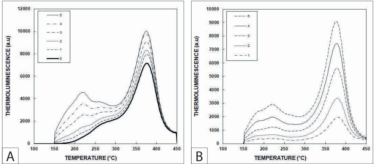
Fig. 9: TL glow-curves of Grand Suc de Breyse maar deposits.
