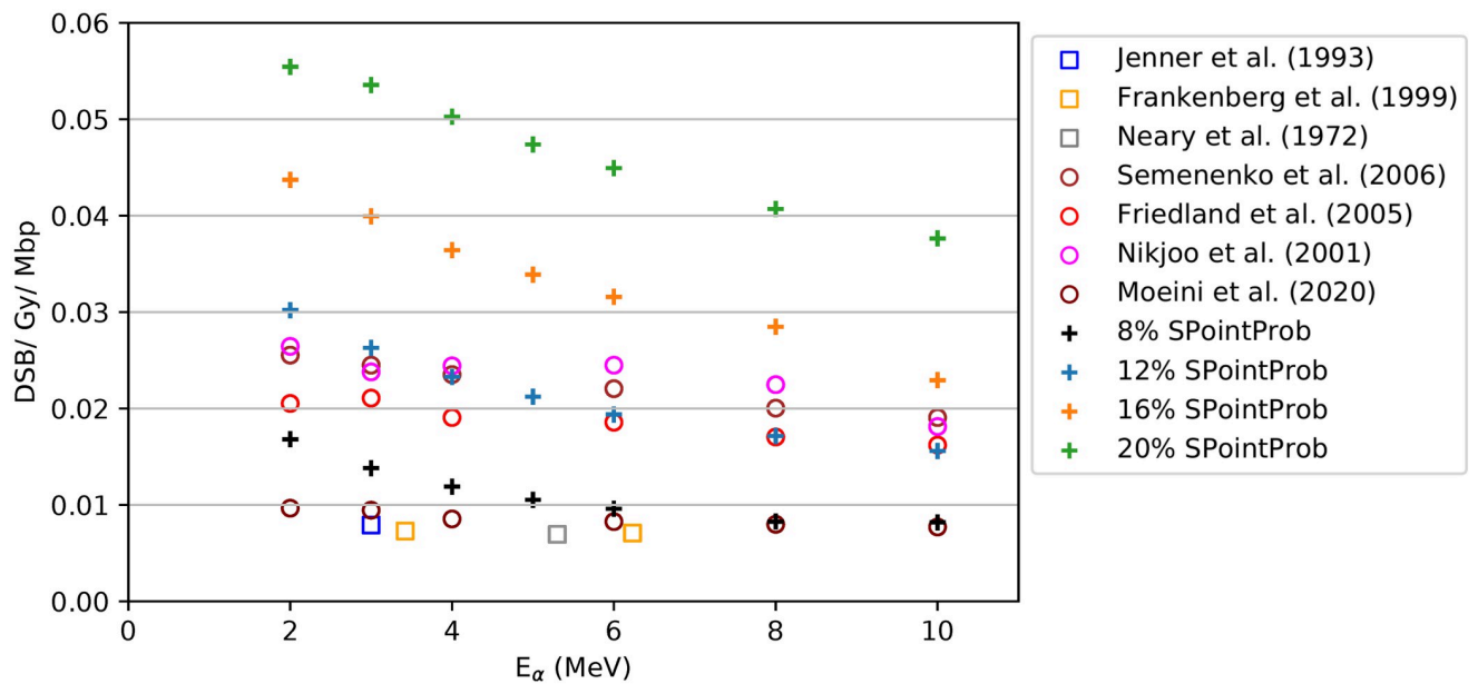
Fig 7. Number of DSB per Gray per Mbp as a function of the energy of \alpha -particles. (+): different values of the SPointProb parameter in our work, ( \circ ): simulations using other codes found in the literature [67–70], ( \square ): experiments found in the literature [71–73].
