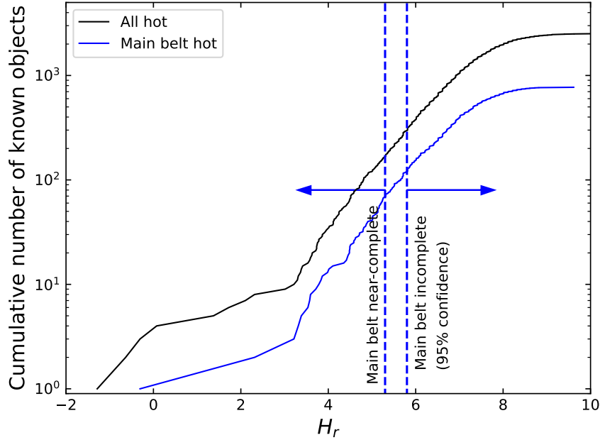
Figure 3. Cumulative H_r distribution (black curve) of all hot TNOs (here, a > 29.5 au and not in the cold population) in the MPC database as of 13 January 2022. The blue curve shows the main-belt subset. The vertical line at H_r = 5.3 represents where our analysis indicates that the the hot main-belt population is nearly complete. The vertical line at H_r = 5.8 shows where the MPC sample is certainly incomplete (95% confidence level). The two samples share very similar H_r distributions brighter than H_r = 5.3 (in particular both distributions show an obviously shallower slope for H_r < 3 ), supporting the claim that all hot objects have the same origin.
