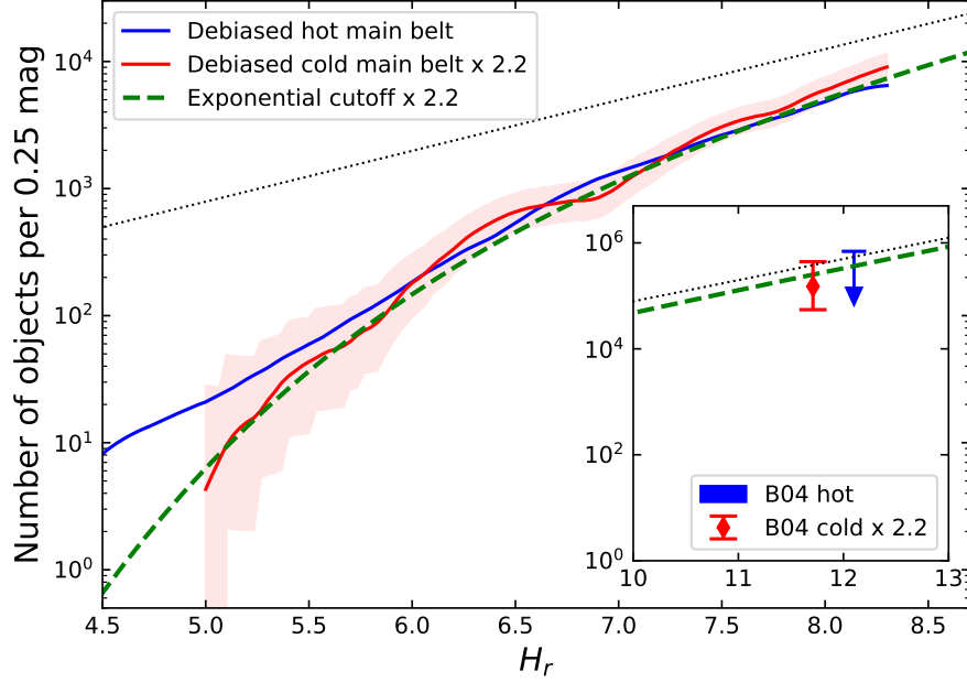
Figure 2. Similar to Fig. 1, where here the debiased cold component estimates and uncertainties have been scaled upward by a factor of 2.2. The green dashed line shows the Kavelaars et al. (2021) cold population exponential cutoff fit (with large- H asymptotic slope of 0.4), also scaled upward by a factor of 2.2. The inset shows the continuation of the scaled exponential cutoff fit at larger/fainter H_r ; the red error-bar gives the 95% confidence range from the detection of three cold TNOs using HST by Bernstein et al. (2004) , and is compatible with the above extrapolation. The inset’s blue arrow shows the 95% confidence upper limit from the non-detection of hot population TNOs in that same HST study. For H_r > 5.5 the shape of the hot and cold population’s are surprisingly similar, which hints at similar formation processes. The black dotted line is a reference exponential with logarithmic slope \alpha = 0.4 , to help see how the exponential taper deviates from a single exponential.
