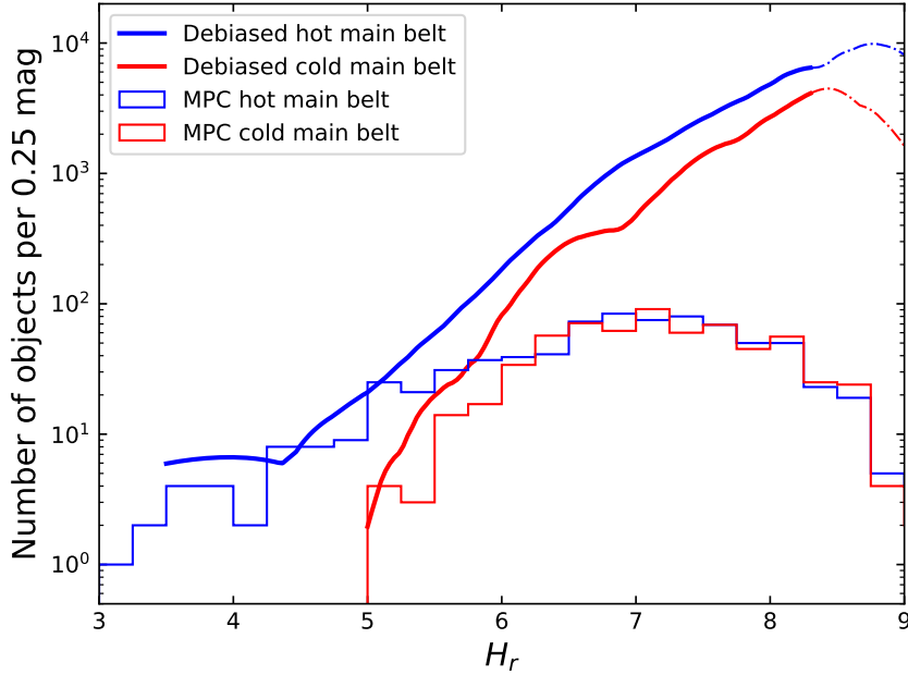
Figure 1. Calibrated differential H_r distribution of the main-belt hot (blue bold curve) and cold (bold red curve) components from debiasing the OSSOS++ sample for H_r \in [3; 8.3] . Less secure estimates (see text) for 8.3 < H_r < 9 , which are only lower limits, are shown by dash-dotted curves. These curves are Epanechnikov Kernel Density Estimates (appendix A) of the debiased H_r absolute magnitude distributions of the main classical belt objects in OSSOS++. The dotted lines represent 95% confidence intervals from Poisson statistics. Up to H_r \simeq 5.3 the OSSOS absolute calibration reproduces the MPC numbers, indicating the latter is now essentially complete in the main-belt.
