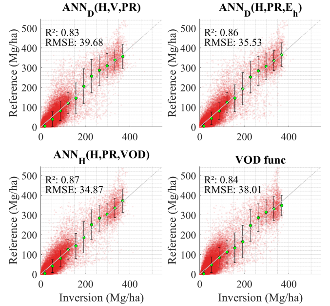
Fig. 9. Scatter plots of the reference AGB (y-axis) with respect to the AGB estimates (x-axis). Uncertainties (represented as black bars) calculated for AGB intervals of 35 Mg/ha. The coefficient of determination and the RMSE (Mg/ha) are shown in the top-left corner of each panel.
