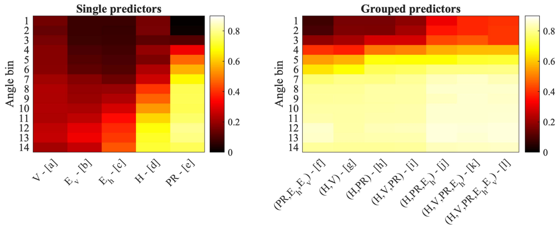
Fig. 2. R^2 values for AGB estimates depending on the angle of incidence (Y-axis) and predictors (X-axis). Bins from 1 to 14 covering angles of incidence between 0^\circ and 65^\circ , in intervals of 5^\circ —see Section II-A. For E , the subindex represents the polarization: E_h corresponds to the horizontal polarization, and E_v to the vertical one. The inversions presented were produced from 2017 datasets using the CCI2017 map as reference.
