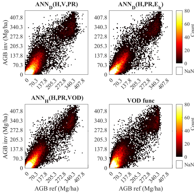
Fig. 7. Heatmap between reference AGB (x-axis) and estimated AGB (y-axis); inversions are produced by models trained with a multiyear dataset and applied to 2018 observation, the reference is the CCI2018 map.
