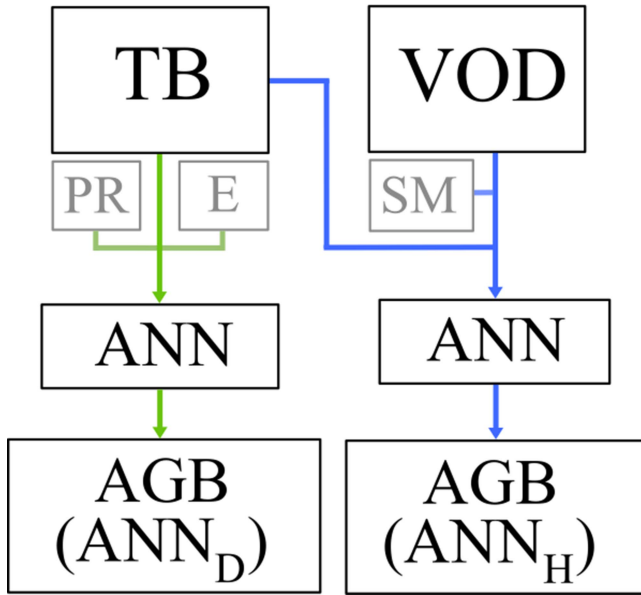
Fig. 1. Sketch of pure data-driven approach ( AGB(ANN_D) ) using TBs or derived variables (like E or PR ) and the hybrid approach ( AGB(ANN_H) ) using TBs and variables from radiative transfer models (VOD or SM).
