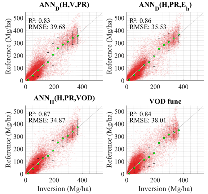
Fig. 9. Scatter plots of the reference AGB (y-axis) with respect to the AGB estimates (x-axis). Uncertainties (represented as black bars) calculated for AGB intervals of 35 Mg/ha. The coefficient of determination and the RMSE (Mg/ha) are shown in the top-left corner of each panel.
