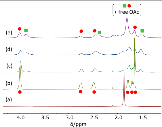
Figure 4. ^1\text{H} NMR spectra, recorded in \text{CD}_2\text{Cl}_2 at 213 K, for solutions of [\text{PPN}]^+\text{OAc}^- (a) and [\text{Rh}(\text{COD})(\mu\text{-OAc})]_2 (30 mg, 0.11 mmol of Rh) in the presence of various amounts of [\text{PPN}]^+\text{OAc}^- (equivalents per Rh atom in parentheses): (b) no added salt; (c) 29 mg (0.049 mmol, 0.44 equiv); (d) 59 mg (0.099 mmol, 0.90 equiv); (e) 81 mg (0.136 mmol, 1.23 equiv). The resonances marked with a red circle belong to [\text{Rh}(\text{COD})(\mu\text{-OAc})]_2 and those marked with a green square to the new species formed in the reaction.
