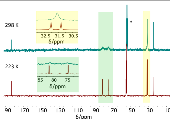
Figure 3. ^{13}\text{C}\{^1\text{H}\} NMR spectra of [\text{Rh}(\text{COD})(\mu\text{-OAc})]_2 in \text{CD}_2\text{Cl}_2 at room temperature and at -50 °C. The starred resonance is due to the solvent.
