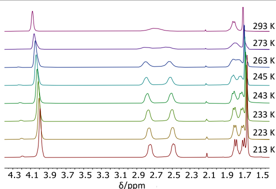
Figure 2. VT ^1\text{H} NMR spectra of [\text{Rh}(\text{COD})(\mu\text{-OAc})]_2 in \text{CD}_2\text{Cl}_2 .
