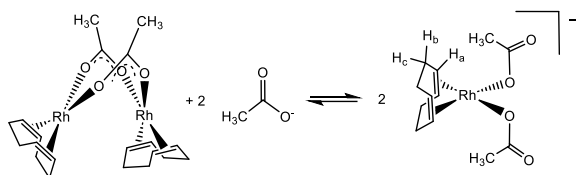
Scheme 3. Equilibrated acetate addition to [\text{Rh}(\text{COD})(\mu\text{-OAc})_2] .
