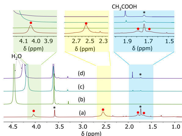
Figure 10. ^1\text{H} NMR spectra, recorded at room temperature in \text{THF-}d_8 , of: (a) [\text{Rh}(\text{COD})(\mu\text{-OAc})]_2 ; (b) the macroRAFT agent \text{R}_0\text{-}[\text{MAA}_{0.5}\text{-co-PEOMA}_{0.5}]_{30}\text{-SC(S)SnPr} ( \text{R}_0 = \text{-C(Me)(CN)CH}_2\text{CH}_2\text{COOH} ); (c) a mixture of macroRAFT agent and [\text{Rh}(\text{COD})(\mu\text{-OAc})]_2 ( \text{MAA}/\text{Rh} = 4 ); (d) same as (c), after spiking with \text{CH}_3\text{COOH} . The starred resonances are due to the residual solvent protons.
