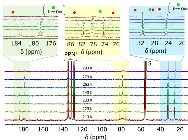
Figure 7. ^{13}\text{C}\{^1\text{H}\} NMR spectra of the solution containing [\text{Rh}(\text{COD})(\mu\text{-OAc})_2] (30 mg) and [\text{PPN}]^+\text{OAc}^- (59 mg, 0.90 equiv per Rh atom) in \text{CD}_2\text{Cl}_2 at different temperatures.
