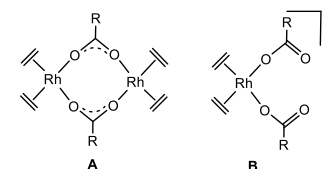
Scheme 1. Structures of known [Rh I (alkene) 2 (O 2 CR)] 2 complexes (A) and of the putative anionic carboxylate adducts, [Rh I (alkene) 2 (O 2 CR) 2 ] - (B).
