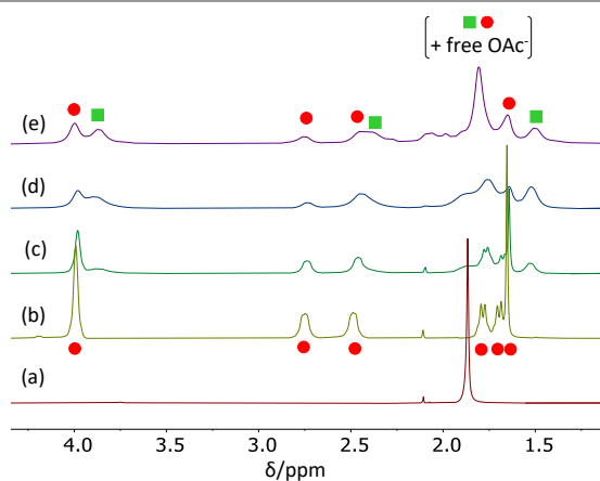
Figure 4. ^1\text{H} NMR spectra, recorded in \text{CD}_2\text{Cl}_2 at 213 K, for solutions of [\text{PPN}]^+\text{OAc}^- (a) and [\text{Rh}(\text{COD})(\mu\text{-OAc})]_2 (30 mg, 0.11 mmol of Rh) in the presence of various amounts of [\text{PPN}]^+\text{OAc}^- (equivalents per Rh atom in parentheses): (b) no added salt; (c) 29 mg (0.049 mmol, 0.44 equiv); (d) 59 mg (0.099 mmol, 0.90 equiv); (e) 81 mg (0.136 mmol, 1.23 equiv). The resonances marked with a red circle belong to [\text{Rh}(\text{COD})(\mu\text{-OAc})]_2 and those marked with a green square to the new species formed in the reaction.
