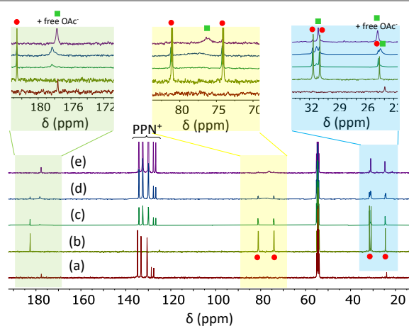
Figure 6. ^{13}\text{C}\{^1\text{H}\} NMR spectra, recorded in \text{CD}_2\text{Cl}_2 at 213 K, for solutions of [\text{PPN}]^+\text{OAc}^- (a) and [\text{Rh}(\text{COD})(\mu\text{-OAc})_2] (30 mg, 0.11 mmol of Rh) in the presence of various amounts of [\text{PPN}]^+\text{OAc}^- (equivalents per Rh atom in parentheses): (b) no added salt; (c) 29 mg (0.049 mmol, 0.44 equiv); (d) 59 mg (0.99 mmol, 0.90 equiv); (e) 81 mg (0.136 mmol, 1.23 equiv). The resonances marked with a red circle belong to [\text{Rh}(\text{COD})(\mu\text{-OAc})_2] and those marked with a green square to the new species formed in the reaction.
