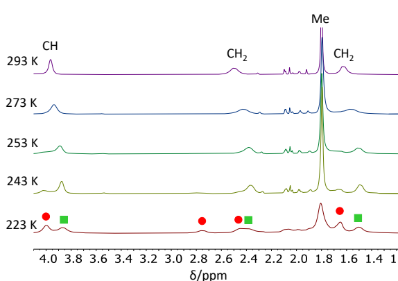
Figure 5. ^1\text{H} NMR spectra of the solution containing [\text{Rh}(\text{COD})(\mu\text{-OAc})_2] (30 mg) and [\text{PPN}]^+\text{OAc}^- (81 mg, 1.23 equiv per Rh atom) in \text{CD}_2\text{Cl}_2 at different temperatures.
