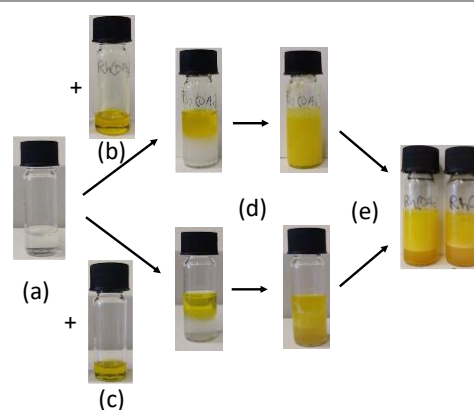
Figure 9. Exposure of toluene solutions of [\text{Rh}(\text{COD})(\mu\text{-OAc})_2] (above) and [\text{Rh}(\text{COD})(\mu\text{-Cl})_2] (below) to an aqueous solution of \text{R}_0\text{-}[\text{MAA}_{0.5}\text{-co-PEOMA}_{0.5}]_{30}\text{-SC(S)SnPr} . (a) Aqueous solution of the macroRAFT agent (90 mmol of COOH functions); (b) [\text{Rh}(\text{COD})(\mu\text{-OAc})_2] (18 mmol of Rh); (c) [\text{Rh}(\text{COD})(\mu\text{-Cl})_2] (18 mmol of Rh); (d) vigorous stirring followed by standing for 5 min; (e) additional vigorous stirring (20 min) followed by standing for 30 min.
