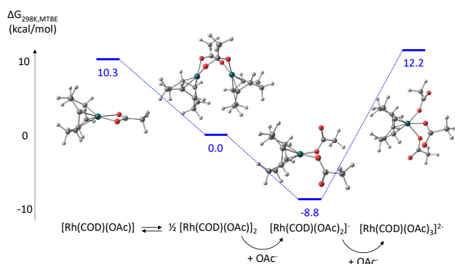
Figure 8. Gibbs energy profile for the [\text{Rh}(\text{COD})(\mu\text{-OAc})_2] dimer/monomer conversion, for the reaction with acetate ions, and for the further acetate addition to [\text{Rh}(\text{COD})(\text{OAc})_2]^- .
