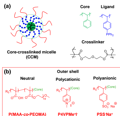
Figure 1. CCM topology (a) and chemical nature of neutral and charged chains in the hydrophilic shell (b).
