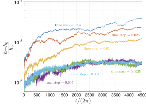
FIG. 10. Mean-value of (h - h_0)/h_0 for an ensemble of guiding-center trajectories as a function of time, computed with different time steps and N = 4096 . The parameters are A = 0.7 , \eta = 0.11 and \rho = 0.3 .
