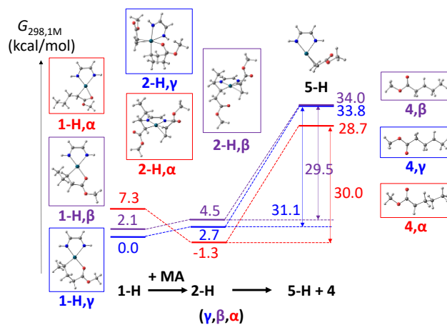
Figure 1. Relative Gibbs energies and views of the optimized geometries for the chelate ring opening by CH 2 =CHCOOMe in 1- H,\alpha/\beta/\gamma and of the Pd-C homolytic bond cleavage in 2- H,\alpha/\beta/\gamma , yielding 4- \alpha/\beta/\gamma and 5- H .
