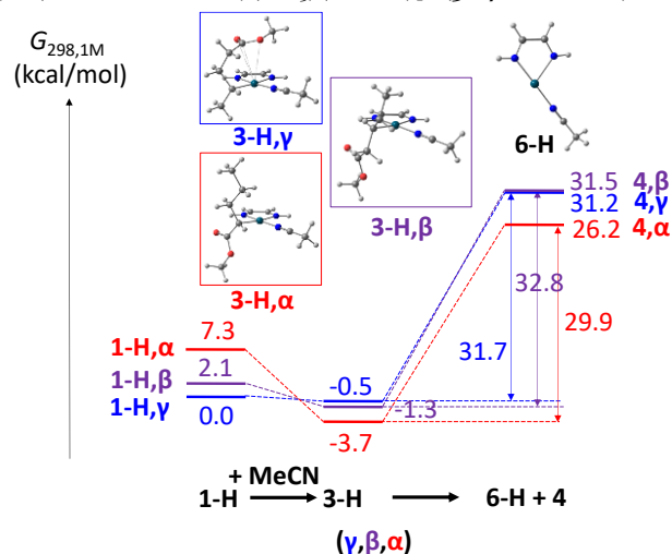
Figure 2. Relative Gibbs energies and views of the optimized geometries for the chelate ring opening by MeCN in 1-H,α/β/γ and of the Pd-C homolytic bond cleavage in 3-H,α/β/γ, yielding 4-α/β/γ and 6-H.
