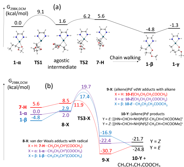
Figure 6. Gibbs energy profile for: (a) the \beta -H elimination process leading from 1-H, \alpha to 7-H ; (b) the H-atom abstraction from the hydride complex 7-H and from the chelated complexes 1-H, \alpha and 1-H, \beta .
