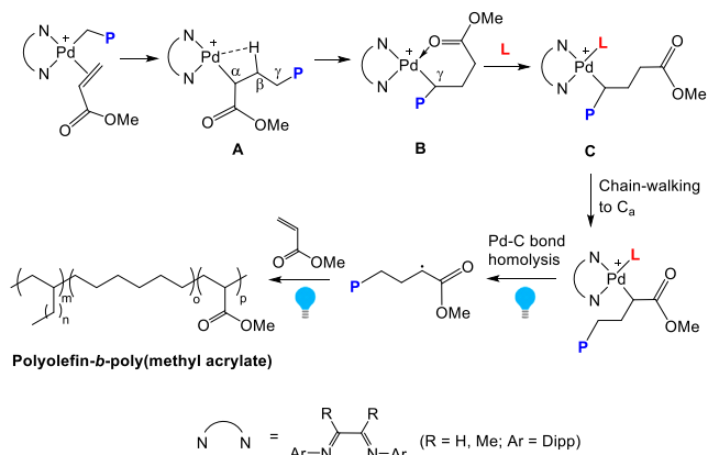
Scheme 1. Chain walking in methyl acrylate/ \alpha -olefin copolymerization catalyzed by cationic ( \alpha -diimine) Pd II complexes and ‘switching’ to the radical pathway (MILRad) to form blockcopolymers
