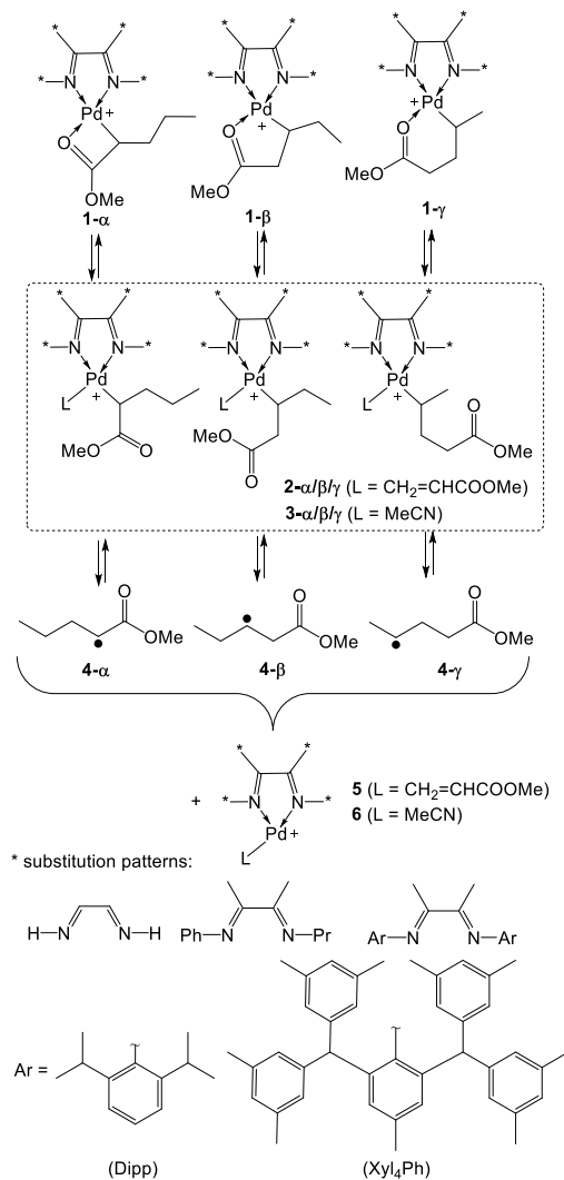
Scheme 4. Systems investigated in this work.
