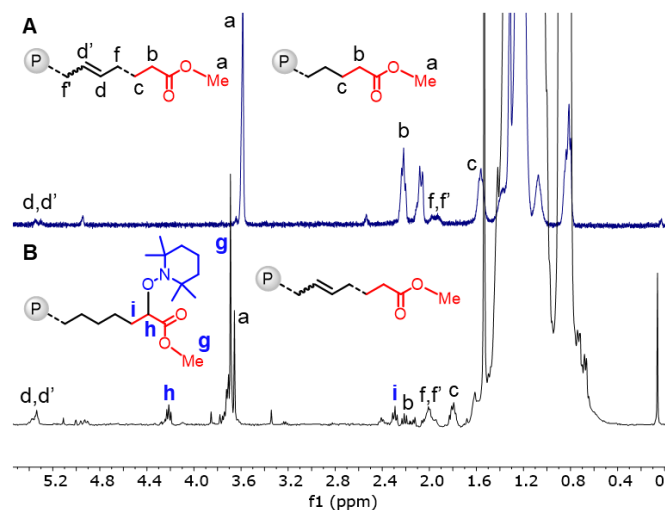
Figure 5. (A) ^1\text{H} NMR of chain-end functionalized PE-MA obtained via thermal activation. (B) ^1\text{H} NMR of TEMPO-trapped PE-MA-TEMPO obtained via light activation.
