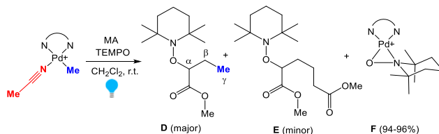
Scheme 2. [\text{Pd}(\text{ArN}=\text{CMeCMe}=\text{NAr})\text{Me}(\text{MeCN})]^+ photolysis in the presence of MA and TEMPO (Ar = Dipp). 13
