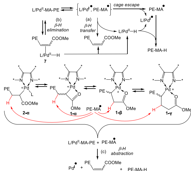
Scheme 5. Possible pathways of Pd-mediated polyacrylate radical disproportionation.
