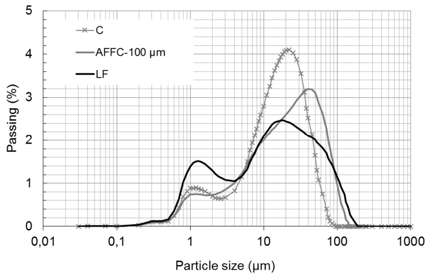
Figure 3. Size distribution of Portland cement (C), limestone filler (LF) and fiber-cement (AFFC-100 µm)
