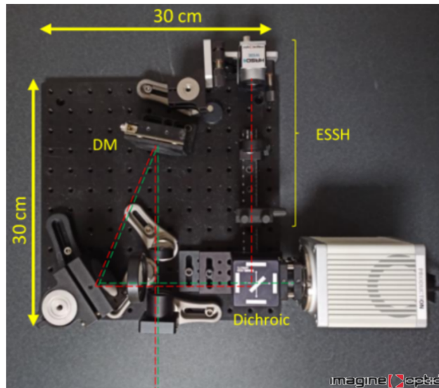
Fig. 5 Compact prototype AO system for LSFM.
