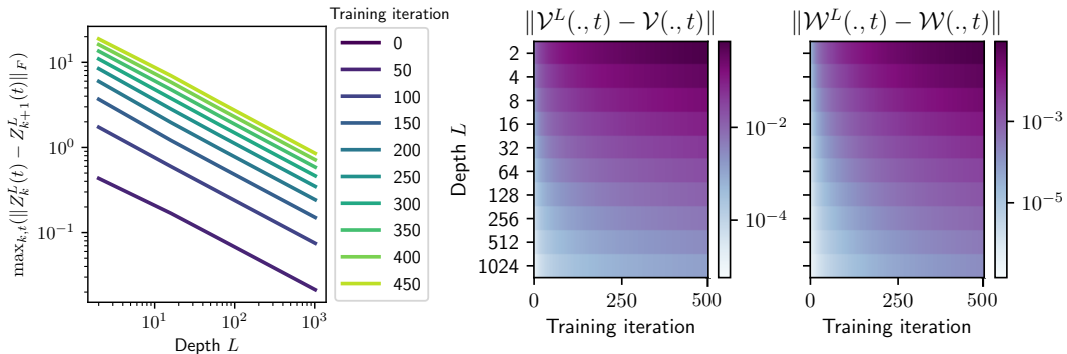
Figure 1: Left: 1/L convergence of the maximum distance between two successive weight matrices \max_{1 \leq k \leq L, t \in [0, T]} (\|Z_k^L(t) - Z_{k+1}^L(t)\|_F) . Right: uniform convergence of \mathcal{Z}^L to its large-depth limit \mathcal{Z} . Here, for a matrix-valued function f , \|f\| denotes (\int_0^1 \|f(s)\|_F^2 ds)^{1/2} .
