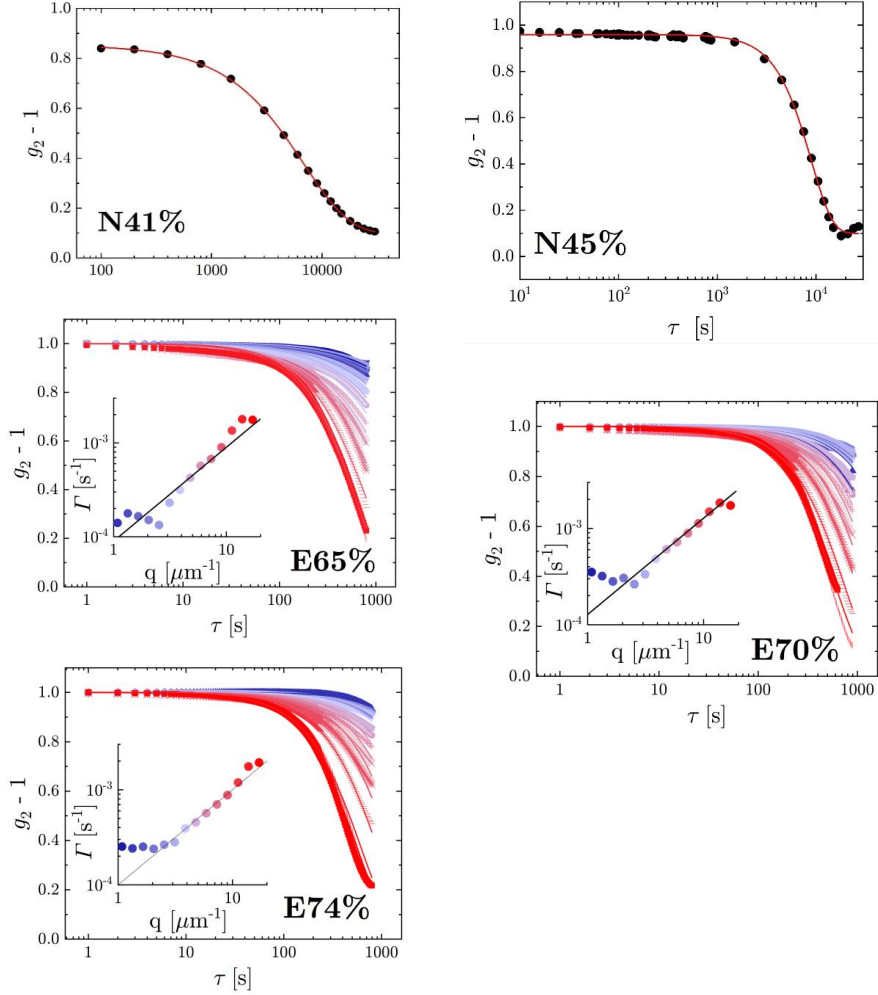
Figure SI5: Dynamics at rest or in the \gamma_0 \rightarrow 0 limit for N and E samples.
