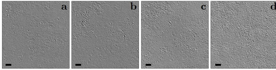
Figure SI16: Coexistence of fast and slow domains as probed by microscopy.
