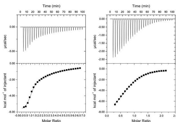
Figure 6: (left) Isothermal Calorimetric Titration data (forward titration) of compound syn-2 in NaOH/H 2 O-KCl buffer (pH = 12.9) at 298 K. The host solution ( c = 0.099 mmol) was placed into the calorimeter cell (1.4 mL) and 28 successive aliquots (10 \mu L) of TIOAc ( c = 3.02 mmol) were added at 3 min intervals (sequential binding site: K_1 = 1.1 \times 10^5 M -1 ; \Delta H_1^0 = -6100 cal.mol -1 ; \Delta S_1^0 = 2.6 cal.mol -1 .K -1 ; \Delta G_1^0 = -6900 cal.mol -1 ; K_2 = 1.8 \times 10^3 M -1 ; \Delta H_2^0 = -15200 cal.mol -1 ; \Delta S_2^0 = -36.1 cal.mol -1 .K -1 ; \Delta G_2^0 = -1100 cal.mol -1 ). (right) Isothermal Calorimetric Titration data (reverse titration) of compound syn-2 recorded in the same conditions. TIOAc ( c = 0.1 mmol) was placed into the calorimeter cell and 28 successive aliquots (10 \mu L) of syn-2 ( c = 0.986 mmol) were added at 3 min intervals ( n = 0.8 ; K = 6.8 \times 10^4 M -1 ; \Delta H^0 = -8900 cal.mol -1 ; \Delta S^0 = -7.8 cal.mol -1 .K -1 ; \Delta G^0 = -6600 cal.mol -1 ).
