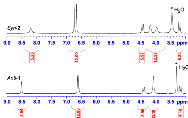
Figure 1: ^1\text{H} NMR spectra of compounds anti-1 and syn-2 recorded in \text{DMSO}-d_6 at 298 K. Full spectrum of syn-2 (0-10 ppm) is reported in Figure S1.
