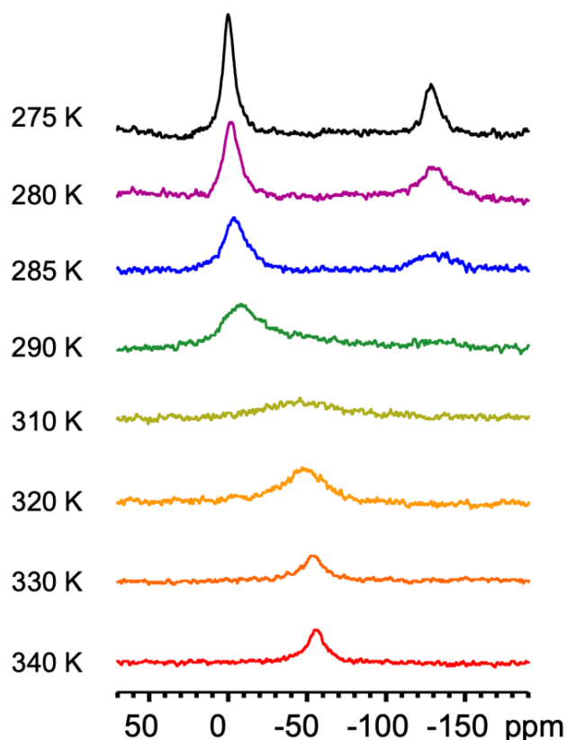
Figure 2: ^{133}\text{Cs} NMR spectra of syn-2 dissolved in NaOD (0.1 M)/ \text{D}_2\text{O} in the presence of an excess of \text{CsNO}_3 . Spectra recorded as a function of temperature (275-340 K).
