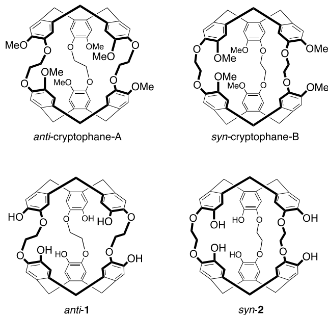
Chart 1: chemical structure of compound anti -cryptophane-A, syn -cryptophane-B, cryptophanes anti -1 and syn -2.
