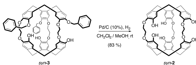
Scheme 1: synthesis of compound syn - 2 from the tris-phenol derivative syn - 3
