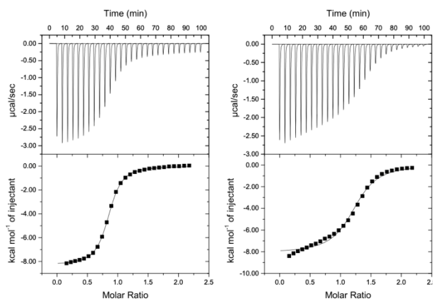
Figure 5: (left) Isothermal Calorimetric Titration data (forward titration) of compound syn-2 in LiOH (0.1 M)/H 2 O at 298 K. The host solution ( c = 0.993 mmol) was placed into the calorimeter cell (1.4 mL) and 28 successive aliquots (10 \mu L) of TIOAc ( c = 0.099 mmol) were added at 3 min intervals ( n = 0.8 ; K = 6.9 \times 10^5 \text{ M}^{-1} ; \Delta H^0 = -8500 \text{ cal.mol}^{-1} ; \Delta S^0 = -1.9 \text{ cal.mol}^{-1}.\text{K}^{-1} ; \Delta G^0 = -7950 \text{ cal.mol}^{-1} ). (right) Isothermal Calorimetric Titration data (reverse titration) of compound syn-2 recorded in the same conditions. TIOAc ( c = 0.10 mmol) was placed into the calorimeter cell and 28 successive aliquots (10 \mu L) of syn-2 ( c = 1.02 mmol) were added at 3 min intervals ( n = 1.2 ; K = 3.25 \times 10^5 \text{ M}^{-1} ; \Delta H^0 = -8100 \text{ cal.mol}^{-1} ; \Delta S^0 = -2.0 \text{ cal.mol}^{-1}.\text{K}^{-1} ; \Delta G^0 = -7500 \text{ cal.mol}^{-1} ).
