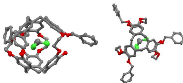
Figure 4: ORTEP representation of compound \text{CH}_2\text{Cl}_2@MP\text{-}syn\text{-}\mathbf{3} . The first stereodescriptor refers to CTB decorated with the three methoxy groups. The Two spatial representations are given for each structure. Hydrogen atoms have been removed for clarity. The displacements ellipsoids were plotted at 30% probability level. In all these structures the ORTEP representation reveals the presence of intra and inter-molecular hydrogen bonding, which have been listed in Tables S4-S5.
