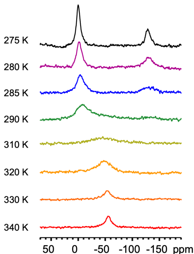
Figure 2: ^{133}\text{Cs} NMR spectra of syn-2 dissolved in NaOD (0.1 M)/D 2 O in the presence of an excess of CsNO 3 . Spectra recorded as a function of temperature (275–340 K).
