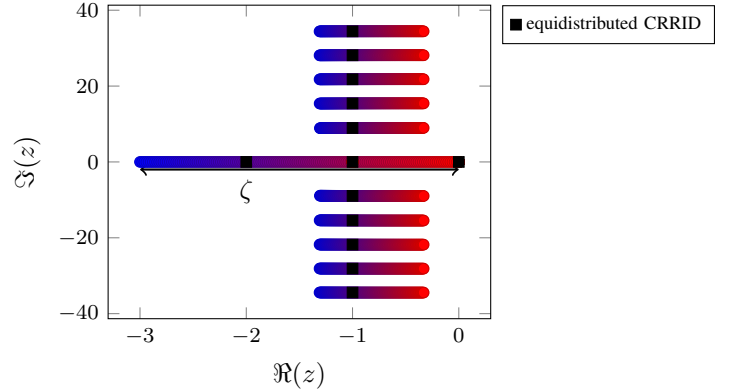
Fig. 1. Spectrum distribution of the normalized quasipolynomial Q for q = 1 and \zeta \in [-3, 0] . The black squares show the spectrum for the case of equidistributed roots z = 0, -1, -2 . The blue color corresponds to \zeta \rightarrow -3 and the red one is for \zeta \rightarrow 0 .
