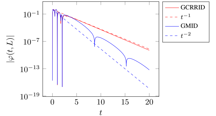
Fig. 3. Comparison of the decay rate of the solutions of (1) with the GCRRID and GMID methods.
