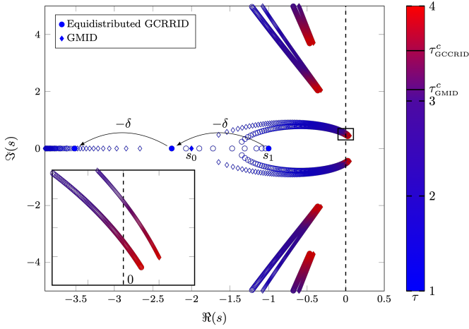
Fig. 4. Migration of the spectrum of the characteristic function (3) with parameters given in (12) in the GCRRID case and in (13) in the GMID case with respect to the perturbation of the delay \tau \in [1, 4] .
