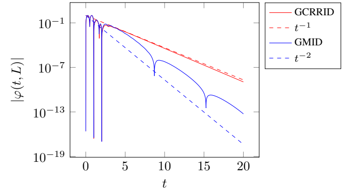
Fig. 3. Comparison of the decay rate of the solutions of (1) with the GCRRID and GMID methods.
