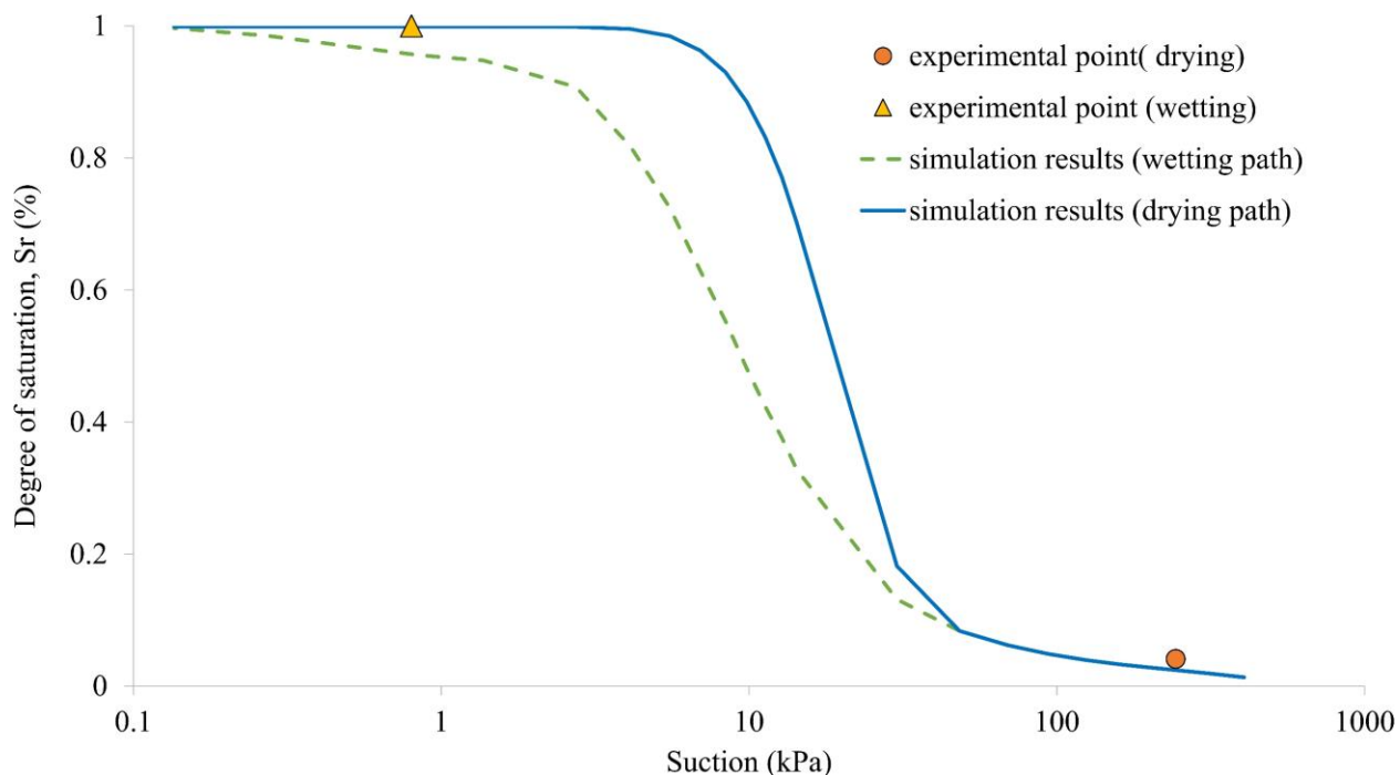
376 377 Fig. 11. Experimental results and simulated results of SWRC on Marche Les Dames Silt 378
