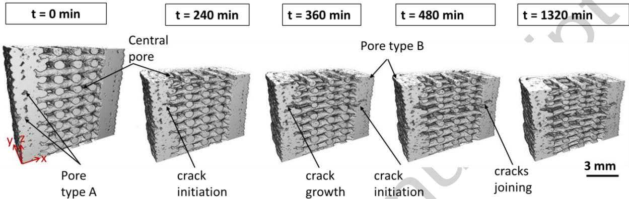
Figure 3: 3D rendered cross-sectional view of reconstructed X-ray tomographic scans at different drying time t
