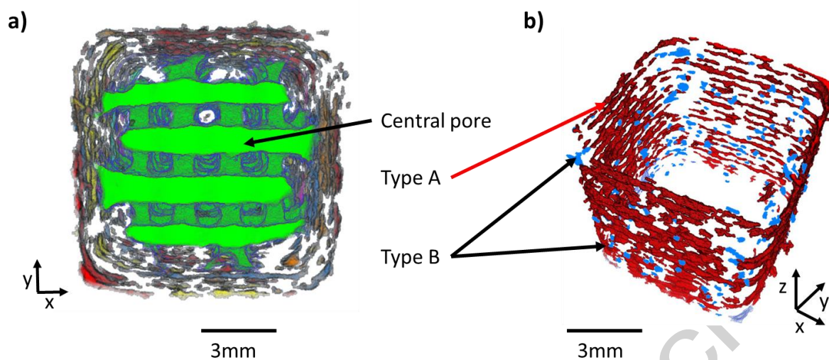
Figure 6: a) 3D rendered view of the sample identifying a) central pore (green), b) type A/intra-filament pores (red) and type B/inter-filaments pores (blue).
