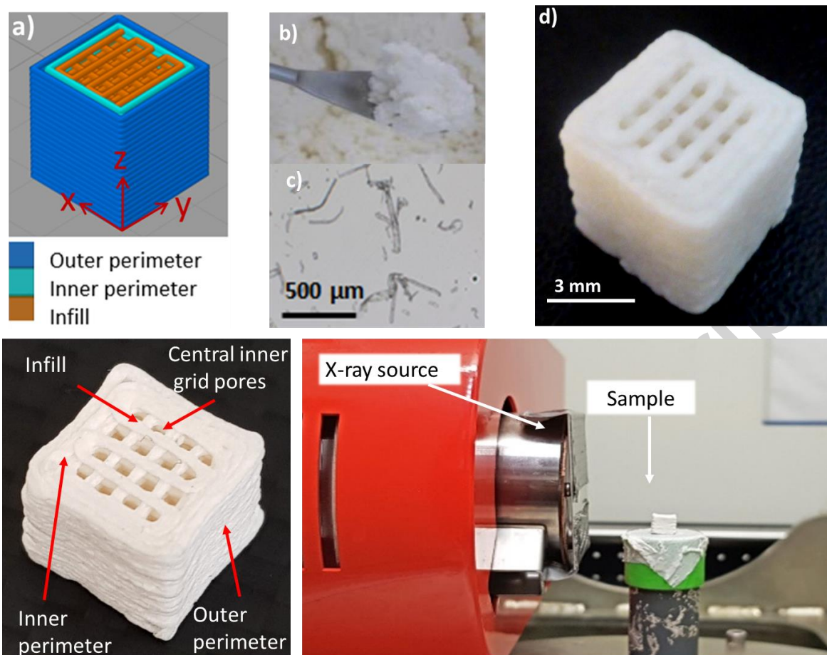
Figure 1: a) 3D STL model of 3D cube to be printed. b) Aqueous carboxymethyl cellulose (CMC) ; c) Natural ligno-cellulosic fibers in suspension; d) Freshly 3D printed cube; e) 3D printed air dried cube; f) Sample placed in the laboratory X-ray microtomograph.
