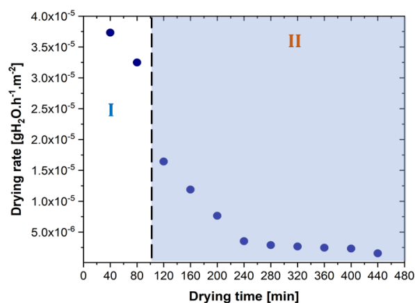
Figure 8: Temporal evolution of the drying rate
