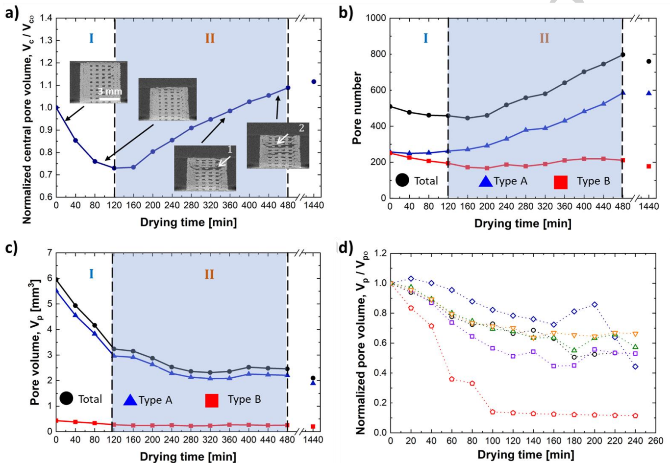
Figure 7: a) Temporal evolution of the deformation of the central pore evolution, where V_{c0} = 94 \text{ mm}^3 , the arrow 1 and 2 indicates the crack formation and the crack joining, respectively b) Temporal evolution of the number of inter-filament porous structures (type pore B) and intra-filament pores (type pores A). c) Temporal evolution of the cumulative volume of inter-filament porous structures (type pore B) and intra-filament of pores (type pores A). d) Normalised pore volume evolution of 6 tracked inter-filament pores; their initial pore volumes are 0.280, 0.249, 0.138, 0.105, 0.094, 0.049 mm 3 for the pore identified by black circle, red diamond, blue diamond, purple square, green triangle and orange triangle, respectively.
