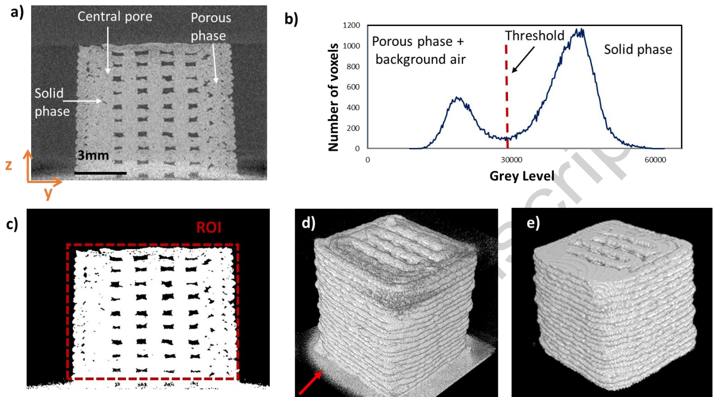
Figure 2: a) Vertical slice of a 3D reconstructed image showing the cube inner structure with porous and solid phases. b) Histogram of reconstructed volume showing the cut-off threshold used to segment the phases. c) Binarized version of the vertical slice (a), with the region of interest (ROI) marked in dashed red lines. d) 3D view of the original binarized volume (solid phase). e) 3D view of working volume.
