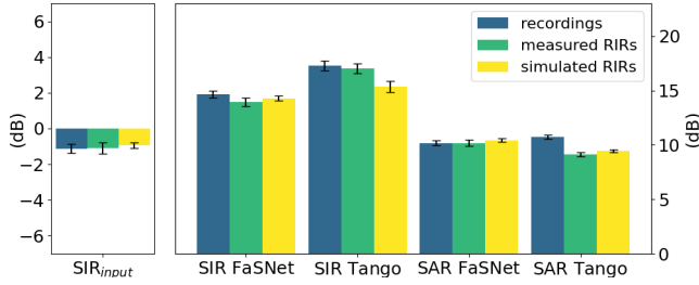
Fig. 2. Mean SE performances obtained for both ears and for all scenarios, on recorded signals, on signals convoluted with measured RIRs and on signals convoluted with simulated RIRs. Signals and RIR measurements are realized with the dummy head.
