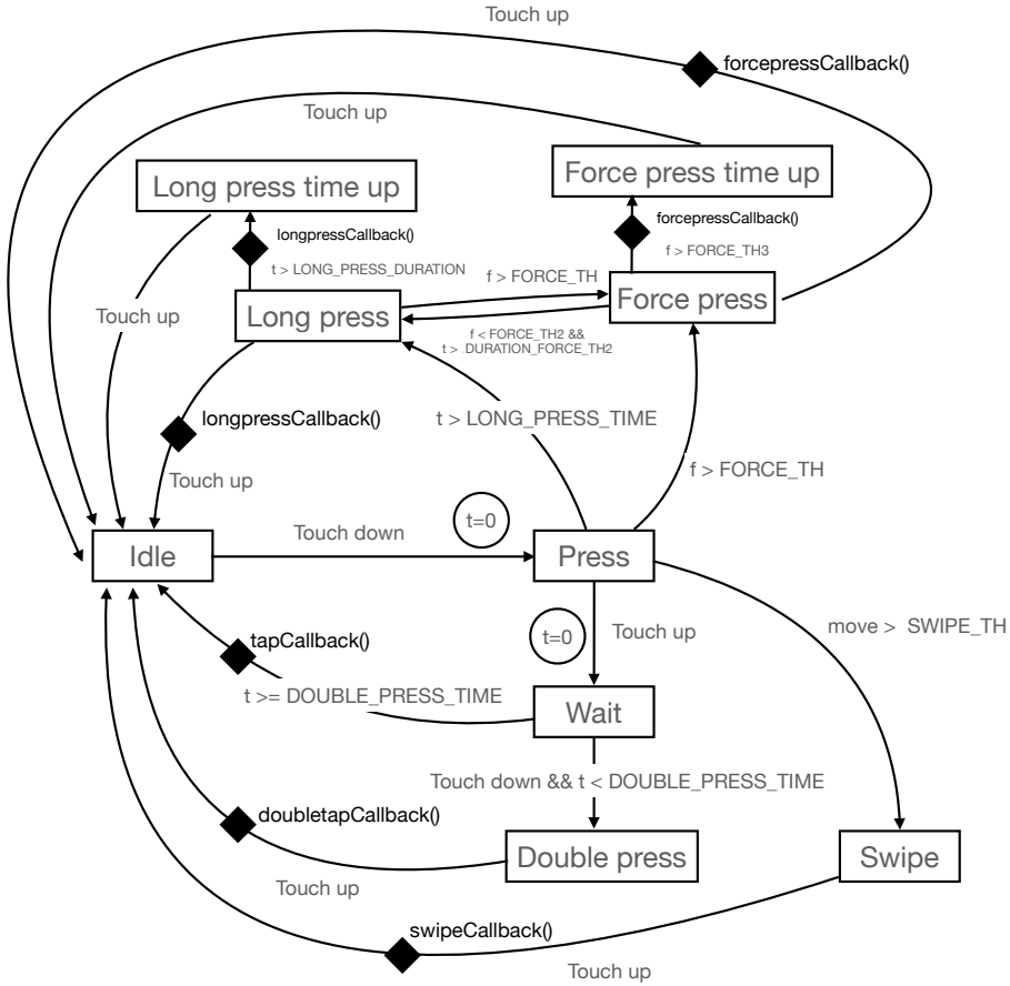
Fig. 10. Finite State Machine used to classify input states in real time during the laboratory experiment. We used the thresholds 0.3s for DOUBLE_PRESS_TIME and 0.75s for LONG_PRESS_DURATION, as defined by default on iOS; 10 pixels for SWIPE_TH; 0.9 for FORCE_TH, 0.7 for FORCE_TH2 and 0.1 s for DURATION_FORCE_TH2. The thresholds for force have arbitrary units but range from 0 to 1 as provided by Pressure.js 2.2.0 and were set using informal tests. Each design is associated with a callback that is considered as correct. Any call to another callback results as an error.
