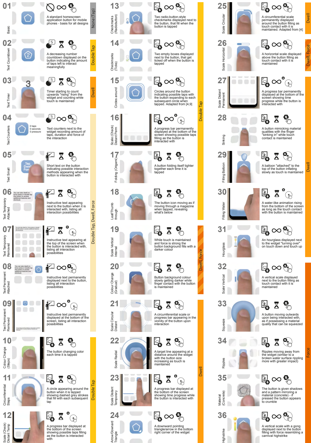
Fig. 4. Table of designs filling the design space. Each design is displayed alongside the design space icons that apply to it and a text description. The vertical strip on the right displays the assumed signified interaction.
