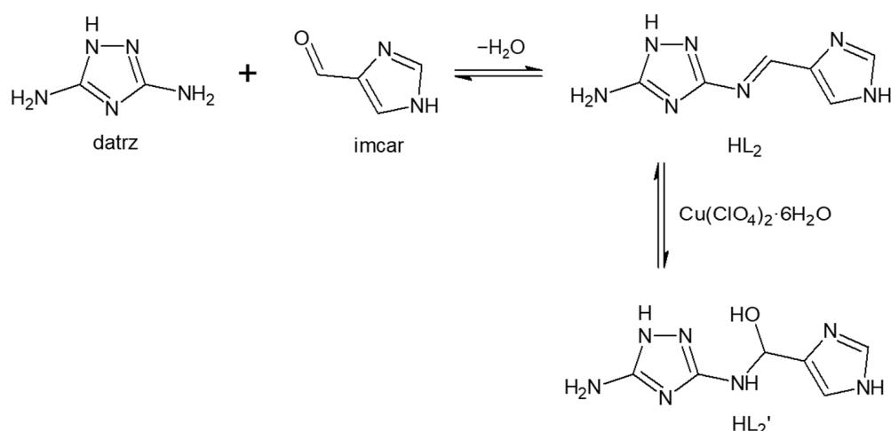
Scheme 1. Proposed synthetic route for ligand H_2L' = [(5\text{-amino-}1H\text{-}1,2,4\text{-triazole-}3\text{-yl)amino}] (1H\text{-}1,2,4\text{-triazol-}4\text{-yl)methanol} ; datz = 1H-1,2,4-triazole-3,5-diamine, Imcar = 1H-imidazole-4-carbaldehyde, H_2L = 3\text{-}[(E)\text{-}[(1H\text{-}1,2,4\text{-triazol-}4\text{-yl)methylidene]amino]\text{-}1H\text{-}1,2,4\text{-triazol-}5\text{-amine} .
